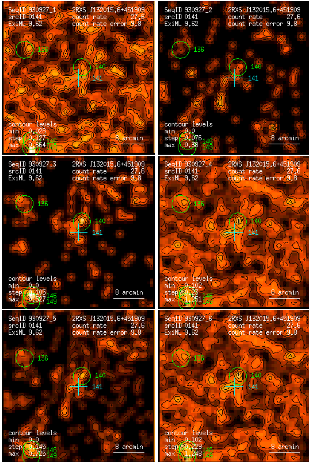
Figure 141: RASS 930927: detection 0141: band rate images, Gaussian filter: (1) PSPC channels 11 – 41, (2) 52 – 90, (3) 91 – 201, (4) 11 – 235, (5) 52 – 201, (6) 11 – 201. Broad band rates in counts/ks. Band rate contour levels in counts/ks/arcmin 2 .
