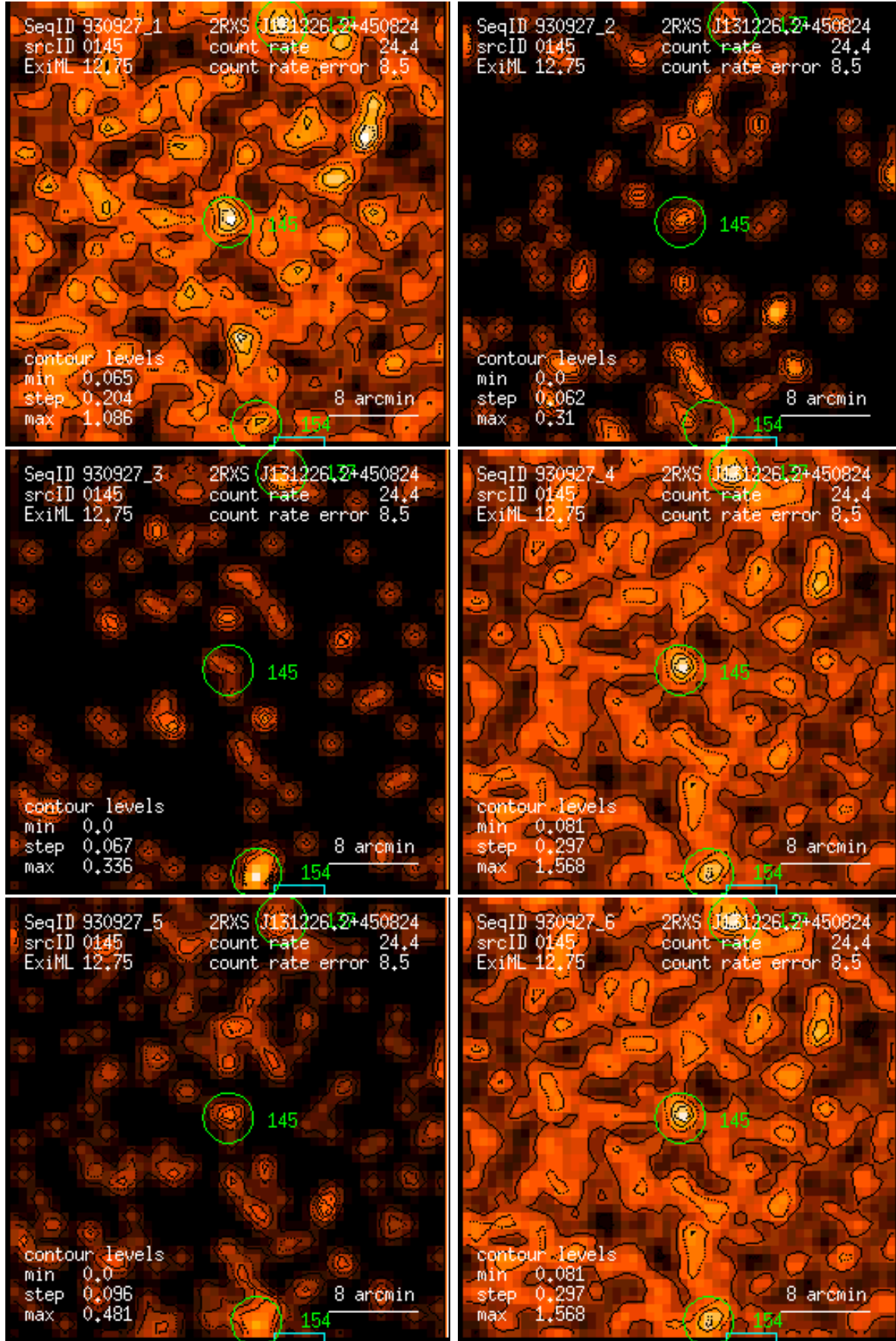
Figure 145: RASS 930927: detection 0145: band rate images, Gaussian filter: (1) PSPC channels 11 – 41, (2) 52 – 90, (3) 91 – 201, (4) 11 – 235, (5) 52 – 201, (6) 11 – 201. Broad band rates in counts/ks. Band rate contour levels in counts/ks/arcmin 2 .
