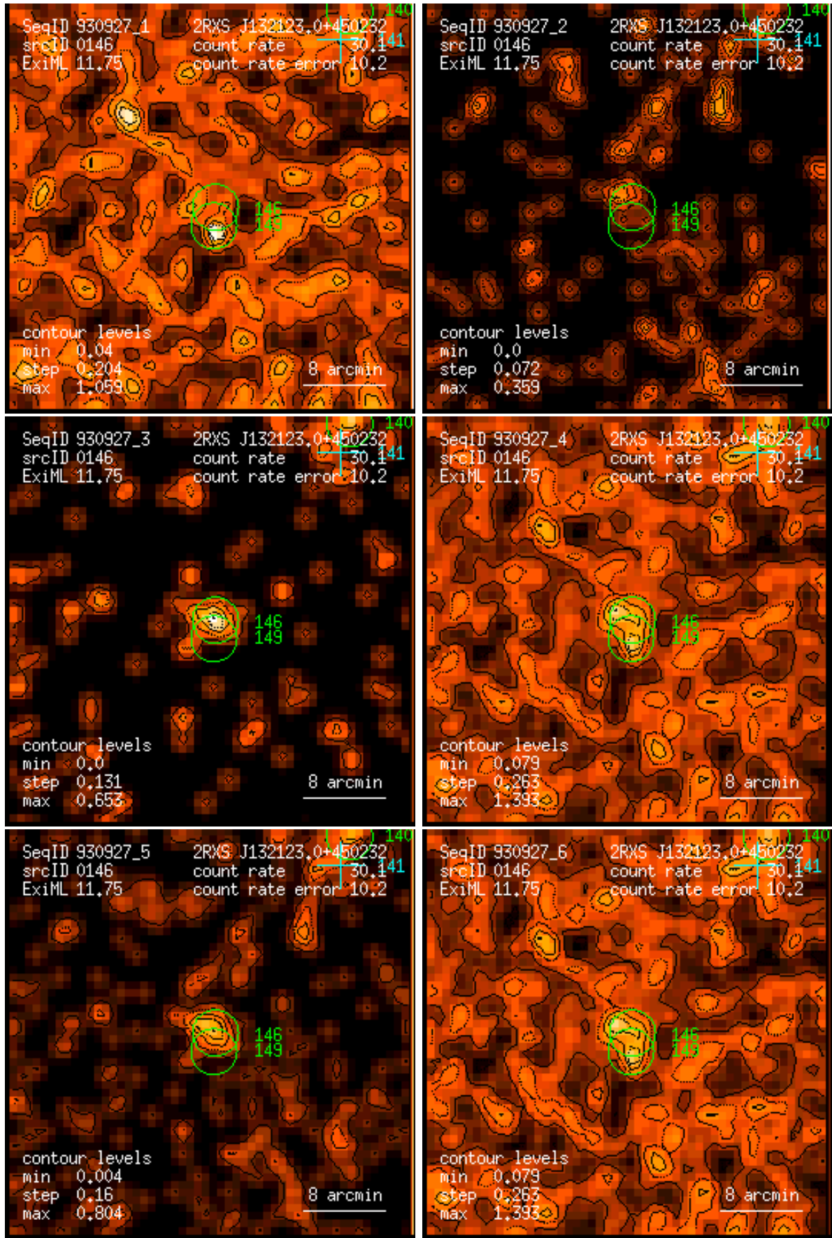
Figure 146: RASS 930927: detection 0146: band rate images, Gaussian filter: (1) PSPC channels 11 – 41, (2) 52 – 90, (3) 91 – 201, (4) 11 – 235, (5) 52 – 201, (6) 11 – 201. Broad band rates in counts/ks. Band rate contour levels in counts/ks/arcmin 2 .
