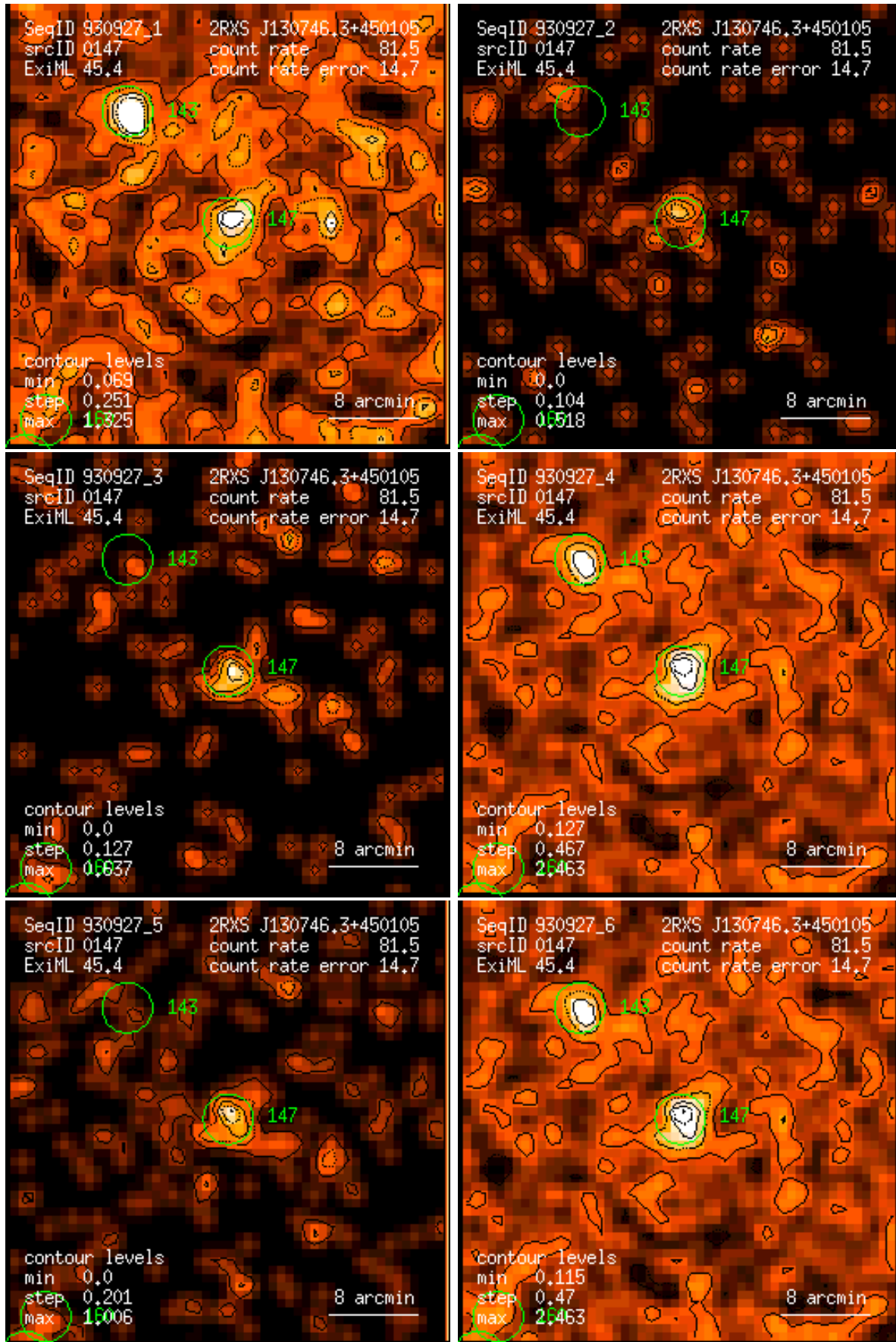
Figure 147: RASS 930927: detection 0147: band rate images, Gaussian filter: (1) PSPC channels 11 – 41, (2) 52 – 90, (3) 91 – 201, (4) 11 – 235, (5) 52 – 201, (6) 11 – 201. Broad band rates in counts/ks. Band rate contour levels in counts/ks/arcmin 2 .
