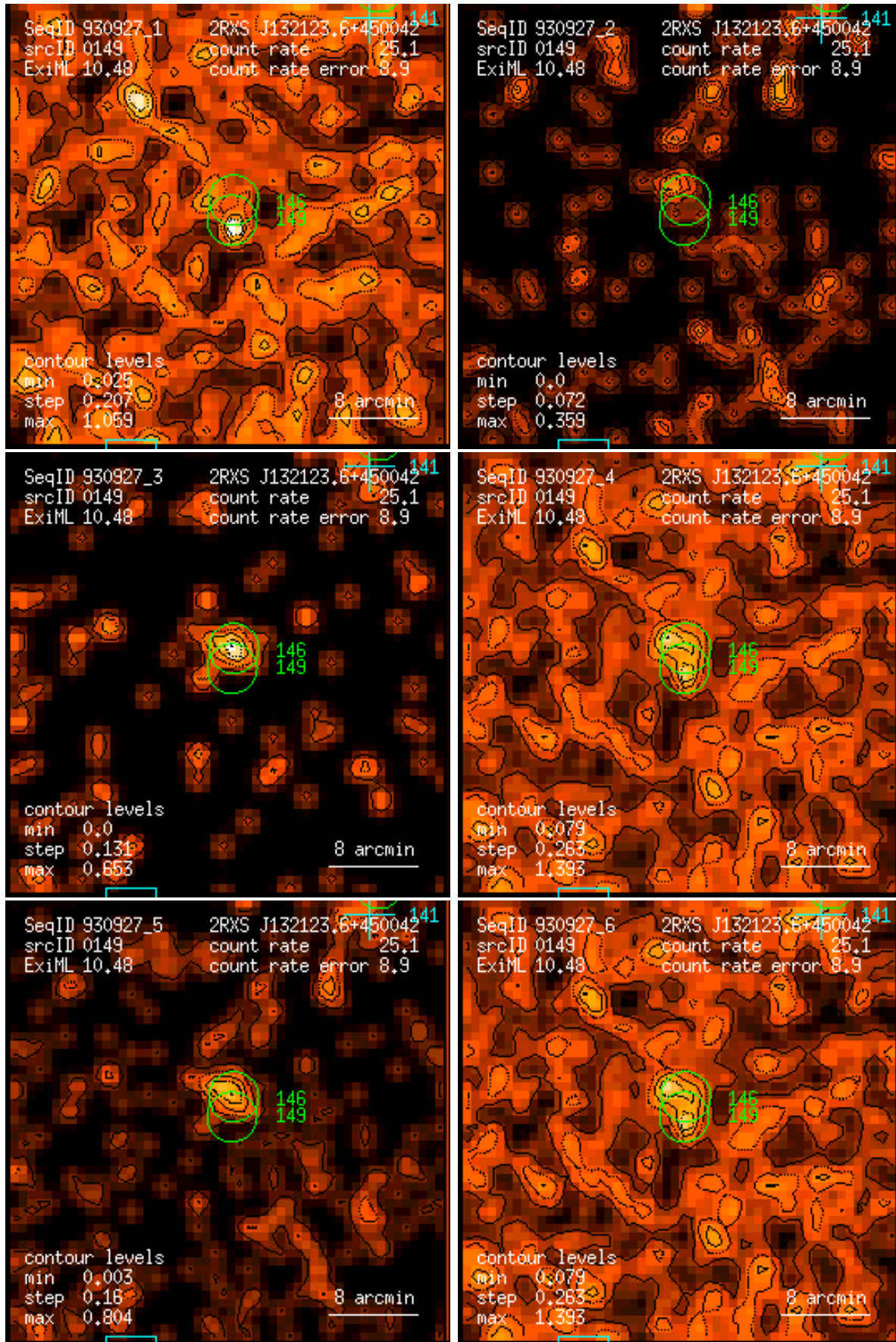
Figure 149: RASS 930927: detection 0149: band rate images, Gaussian filter: (1) PSPC channels 11 – 41, (2) 52 – 90, (3) 91 – 201, (4) 11 – 235, (5) 52 – 201, (6) 11 – 201. Broad band rates in counts/ks. Band rate contour levels in counts/ks/arcmin 2 .
