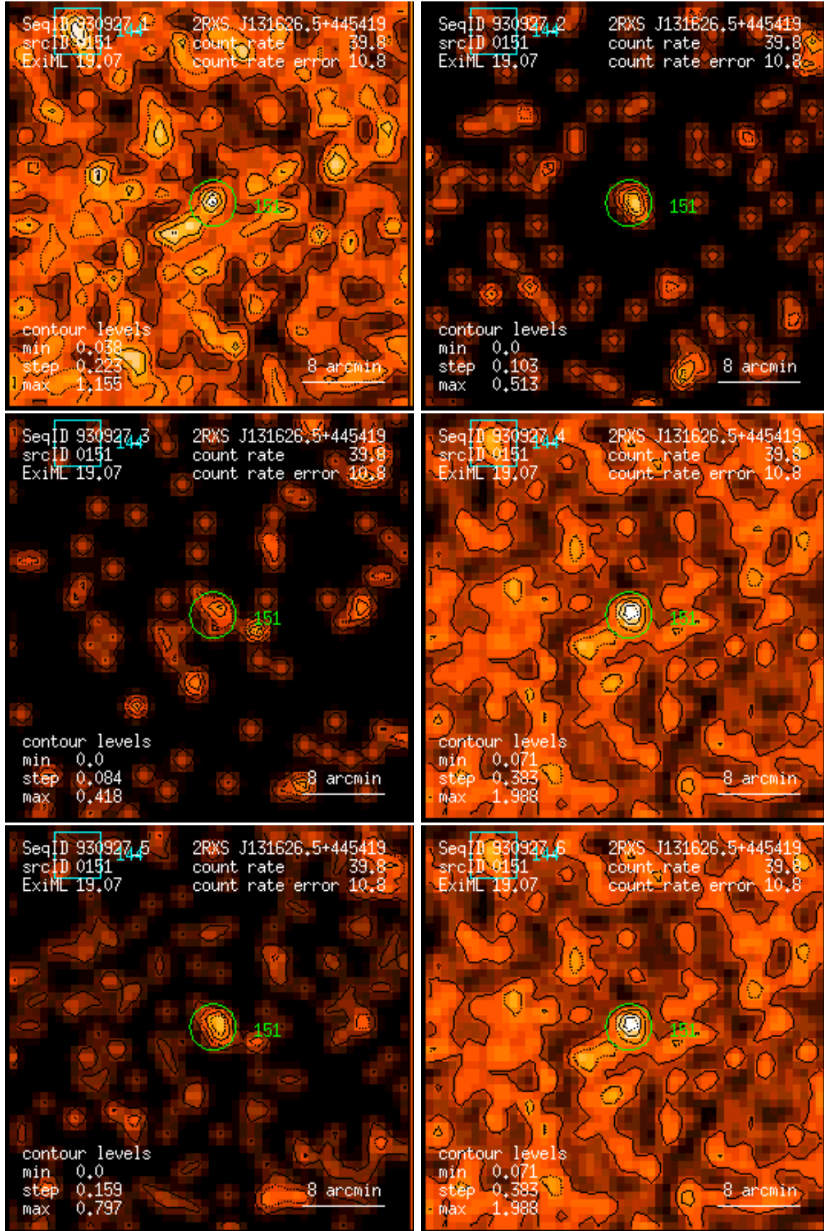
Figure 151: RASS 930927: detection 0151: band rate images, Gaussian filter: (1) PSPC channels 11 – 41, (2) 52 – 90, (3) 91 – 201, (4) 11 – 235, (5) 52 – 201, (6) 11 – 201. Broad band rates in counts/ks. Band rate contour levels in counts/ks/arcmin 2 .
