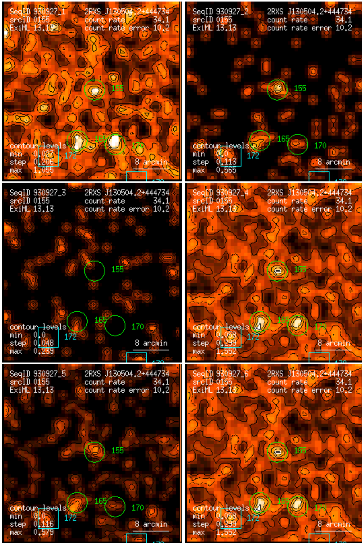
Figure 155: RASS 930927: detection 0155: band rate images, Gaussian filter: (1) PSPC channels 11 – 41, (2) 52 – 90, (3) 91 – 201, (4) 11 – 235, (5) 52 – 201, (6) 11 – 201. Broad band rates in counts/ks. Band rate contour levels in counts/ks/arcmin 2 .
