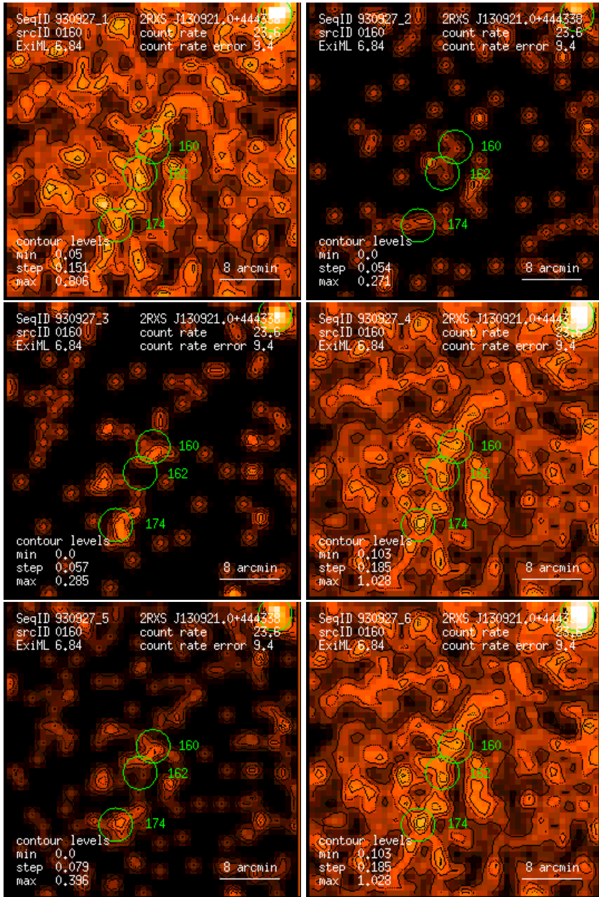
Figure 160: RASS 930927: detection 0160: band rate images, Gaussian filter: (1) PSPC channels 11 – 41, (2) 52 – 90, (3) 91 – 201, (4) 11 – 235, (5) 52 – 201, (6) 11 – 201. Broad band rates in counts/ks. Band rate contour levels in counts/ks/arcmin 2 .
