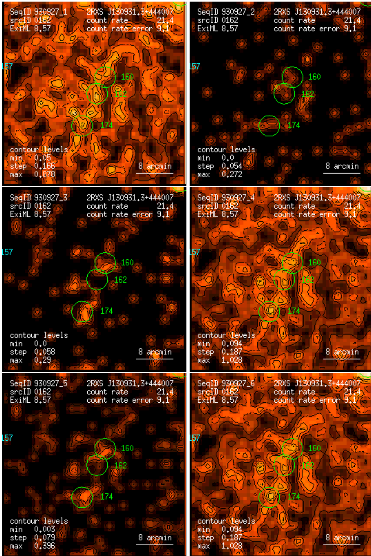
Figure 162: RASS 930927: detection 0162: band rate images, Gaussian filter: (1) PSPC channels 11 – 41, (2) 52 – 90, (3) 91 – 201, (4) 11 – 235, (5) 52 – 201, (6) 11 – 201. Broad band rates in counts/ks. Band rate contour levels in counts/ks/arcmin 2 .
