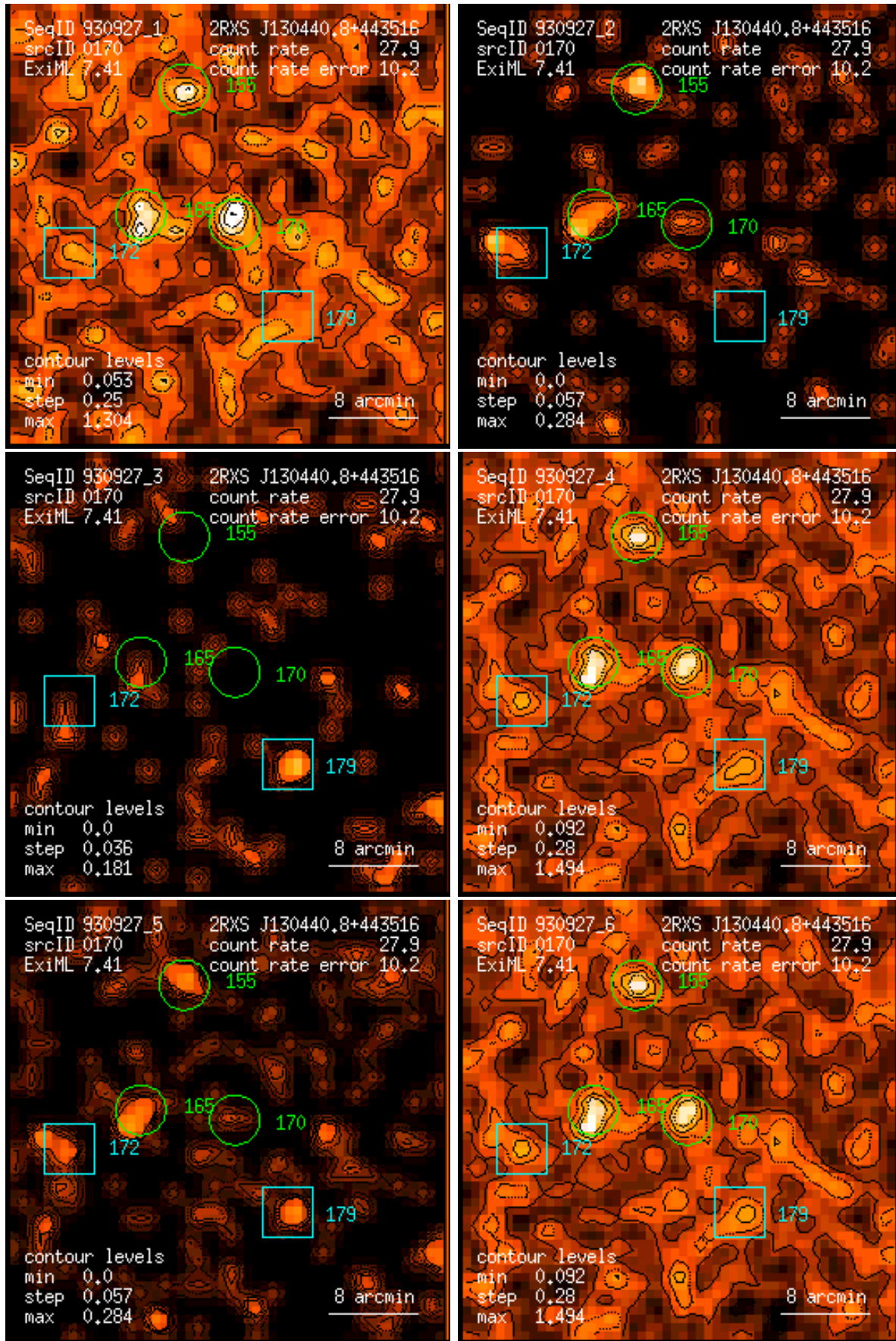
Figure 170: RASS 930927: detection 0170: band rate images, Gaussian filter: (1) PSPC channels 11 – 41, (2) 52 – 90, (3) 91 – 201, (4) 11 – 235, (5) 52 – 201, (6) 11 – 201. Broad band rates in counts/ks. Band rate contour levels in counts/ks/arcmin 2 .
