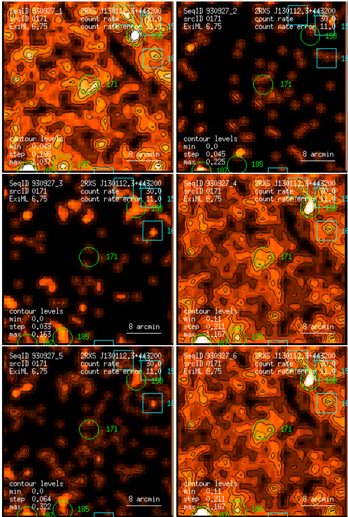
Figure 171: RASS 930927: detection 0171: band rate images, Gaussian filter: (1) PSPC channels 11 – 41, (2) 52 – 90, (3) 91 – 201, (4) 11 – 235, (5) 52 – 201, (6) 11 – 201. Broad band rates in counts/ks. Band rate contour levels in counts/ks/arcmin 2 .
