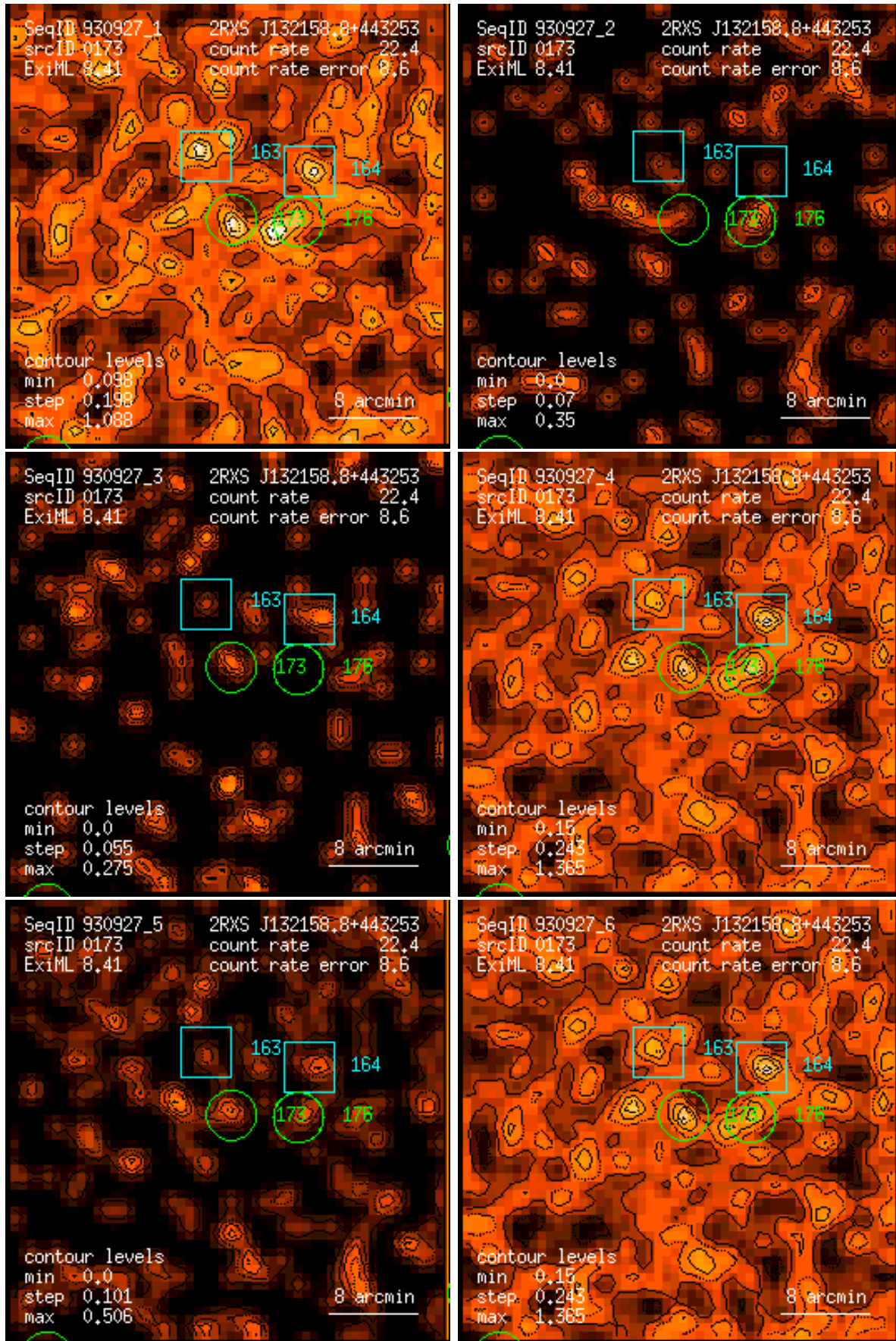
Figure 173: RASS 930927: detection 0173: band rate images, Gaussian filter: (1) PSPC channels 11 – 41, (2) 52 – 90, (3) 91 – 201, (4) 11 – 235, (5) 52 – 201, (6) 11 – 201. Broad band rates in counts/ks. Band rate contour levels in counts/ks/arcmin 2 .
