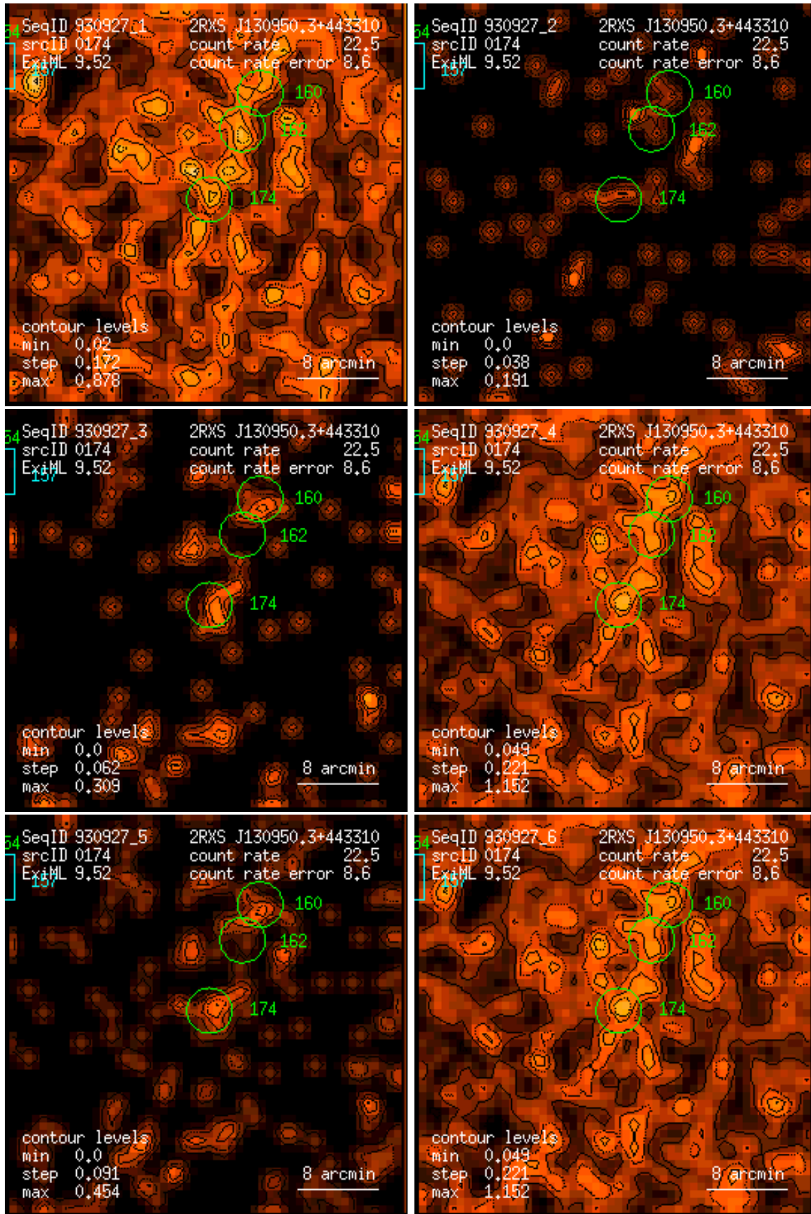
Figure 174: RASS 930927: detection 0174: band rate images, Gaussian filter: (1) PSPC channels 11 – 41, (2) 52 – 90, (3) 91 – 201, (4) 11 – 235, (5) 52 – 201, (6) 11 – 201. Broad band rates in counts/ks. Band rate contour levels in counts/ks/arcmin 2 .
