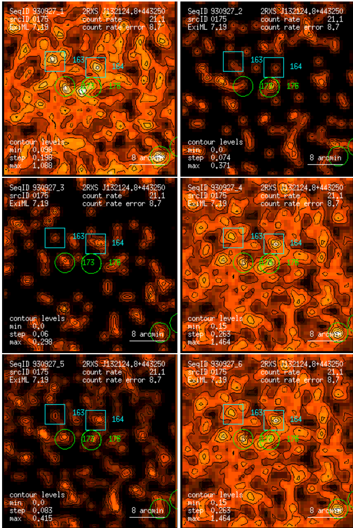
Figure 175: RASS 930927: detection 0175: band rate images, Gaussian filter: (1) PSPC channels 11 – 41, (2) 52 – 90, (3) 91 – 201, (4) 11 – 235, (5) 52 – 201, (6) 11 – 201. Broad band rates in counts/ks. Band rate contour levels in counts/ks/arcmin 2 .
