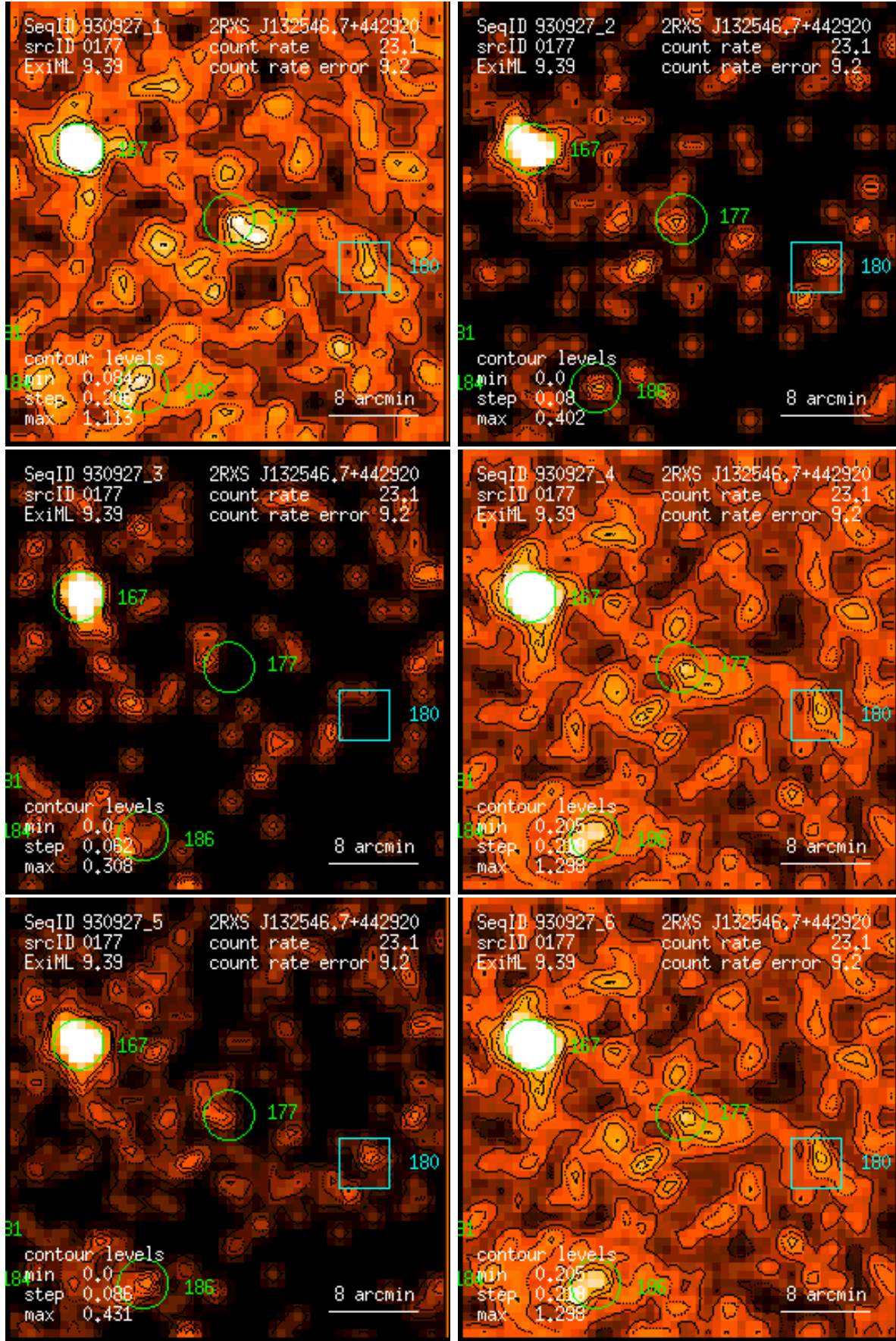
Figure 177: RASS 930927: detection 0177: band rate images, Gaussian filter: (1) PSPC channels 11 – 41, (2) 52 – 90, (3) 91 – 201, (4) 11 – 235, (5) 52 – 201, (6) 11 – 201. Broad band rates in counts/ks. Band rate contour levels in counts/ks/arcmin 2 .
