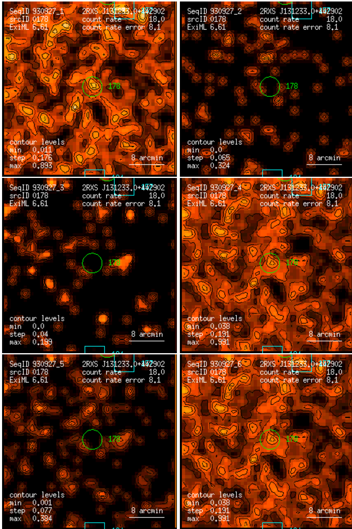
Figure 178: RASS 930927: detection 0178: band rate images, Gaussian filter: (1) PSPC channels 11 – 41, (2) 52 – 90, (3) 91 – 201, (4) 11 – 235, (5) 52 – 201, (6) 11 – 201. Broad band rates in counts/ks. Band rate contour levels in counts/ks/arcmin 2 .
