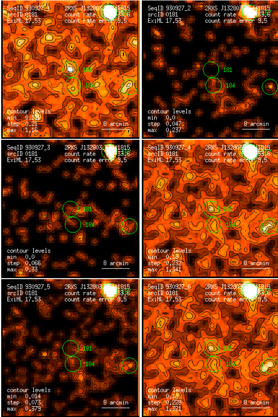
Figure 181: RASS 930927: detection 0181: band rate images, Gaussian filter: (1) PSPC channels 11 – 41, (2) 52 – 90, (3) 91 – 201, (4) 11 – 235, (5) 52 – 201, (6) 11 – 201. Broad band rates in counts/ks. Band rate contour levels in counts/ks/arcmin 2 .
