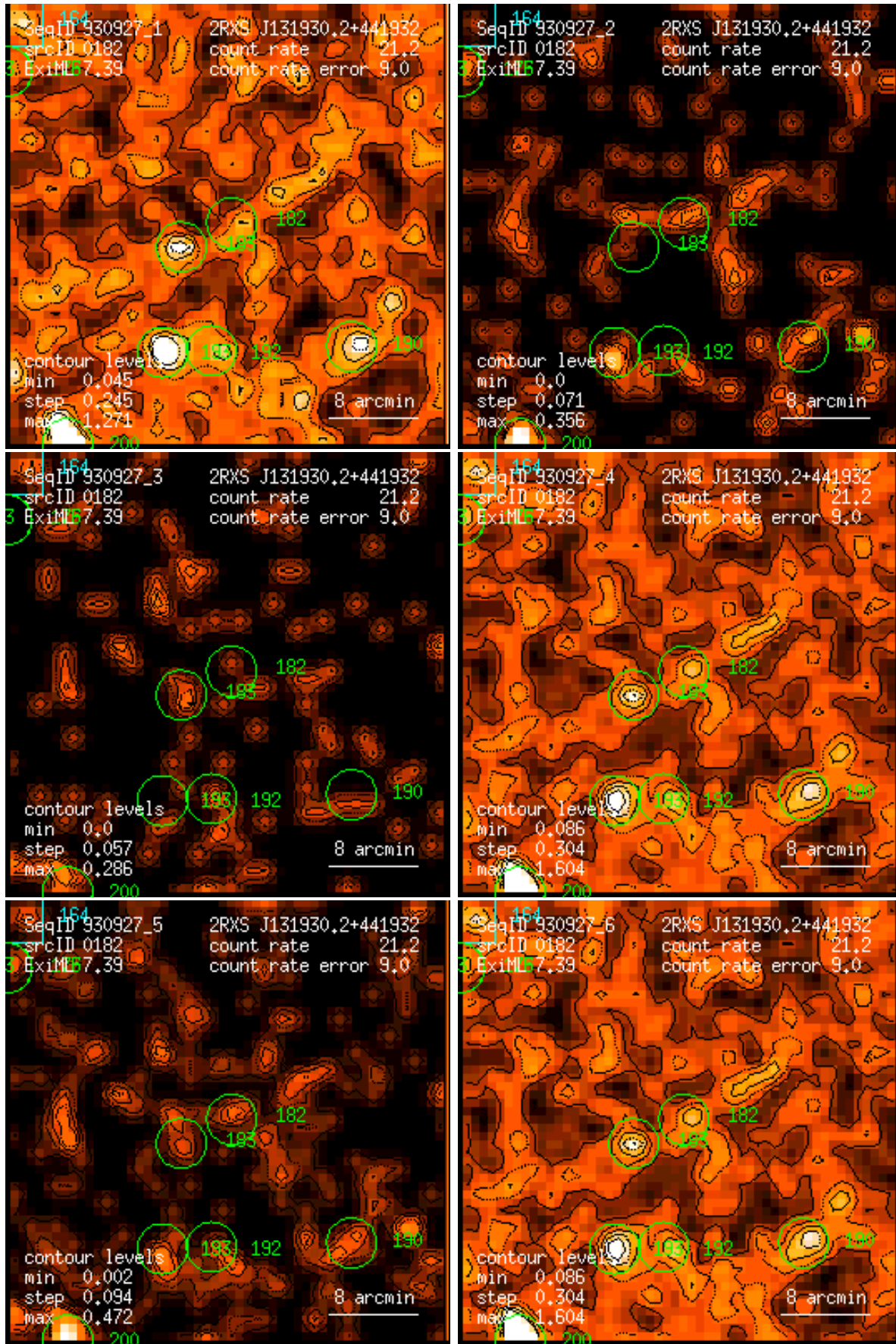
Figure 182: RASS 930927: detection 0182: band rate images, Gaussian filter: (1) PSPC channels 11 – 41, (2) 52 – 90, (3) 91 – 201, (4) 11 – 235, (5) 52 – 201, (6) 11 – 201. Broad band rates in counts/ks. Band rate contour levels in counts/ks/arcmin 2 .
