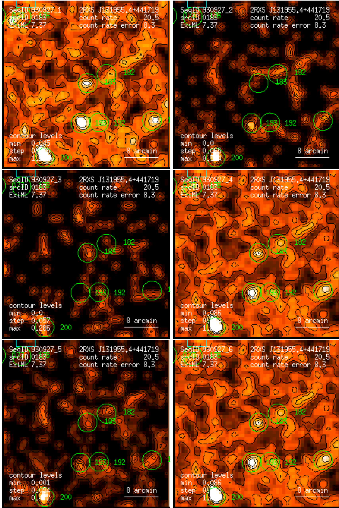
Figure 183: RASS 930927: detection 0183: band rate images, Gaussian filter: (1) PSPC channels 11 – 41, (2) 52 – 90, (3) 91 – 201, (4) 11 – 235, (5) 52 – 201, (6) 11 – 201. Broad band rates in counts/ks. Band rate contour levels in counts/ks/arcmin 2 .
