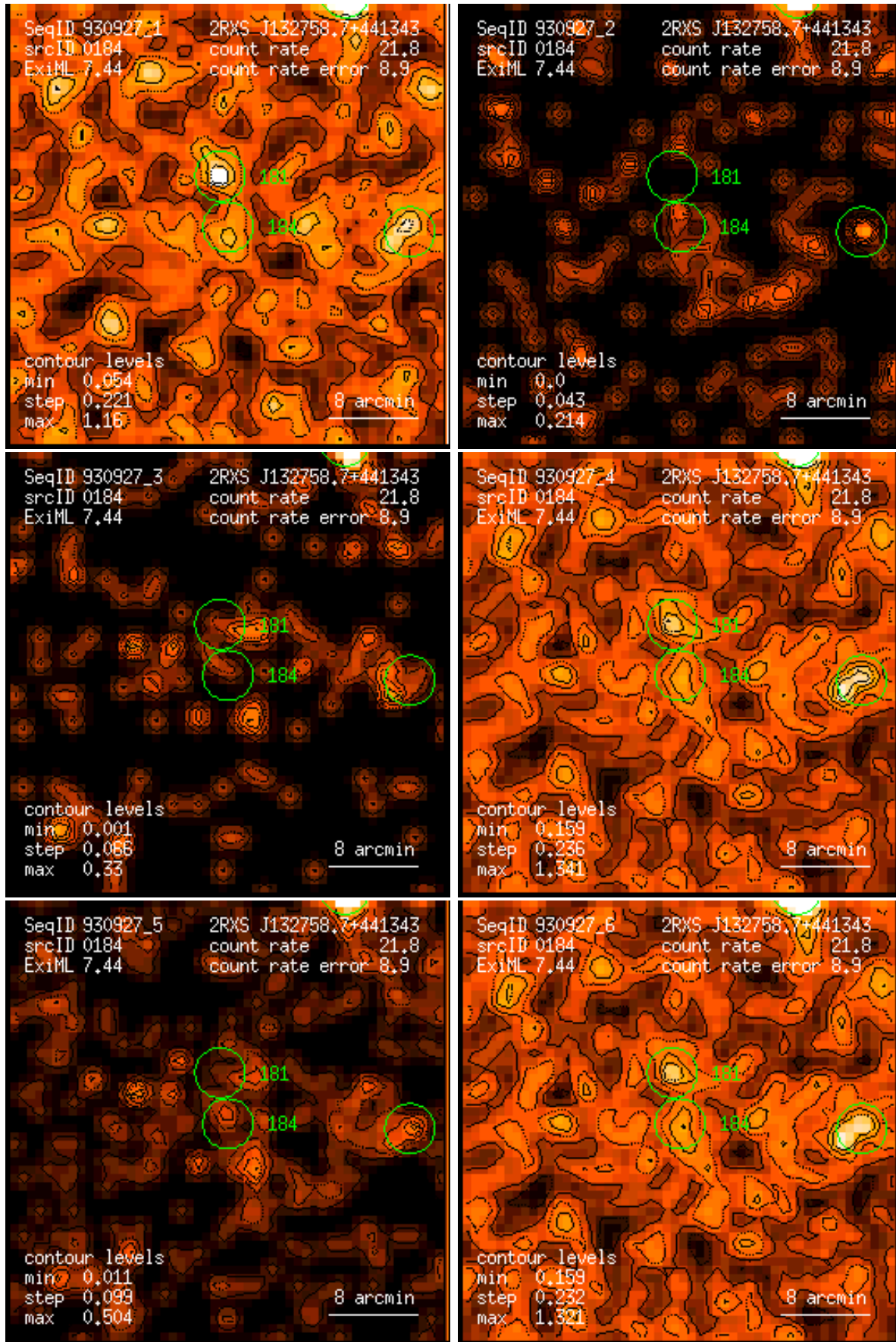
Figure 184: RASS 930927: detection 0184: band rate images, Gaussian filter: (1) PSPC channels 11 – 41, (2) 52 – 90, (3) 91 – 201, (4) 11 – 235, (5) 52 – 201, (6) 11 – 201. Broad band rates in counts/ks. Band rate contour levels in counts/ks/arcmin 2 .
