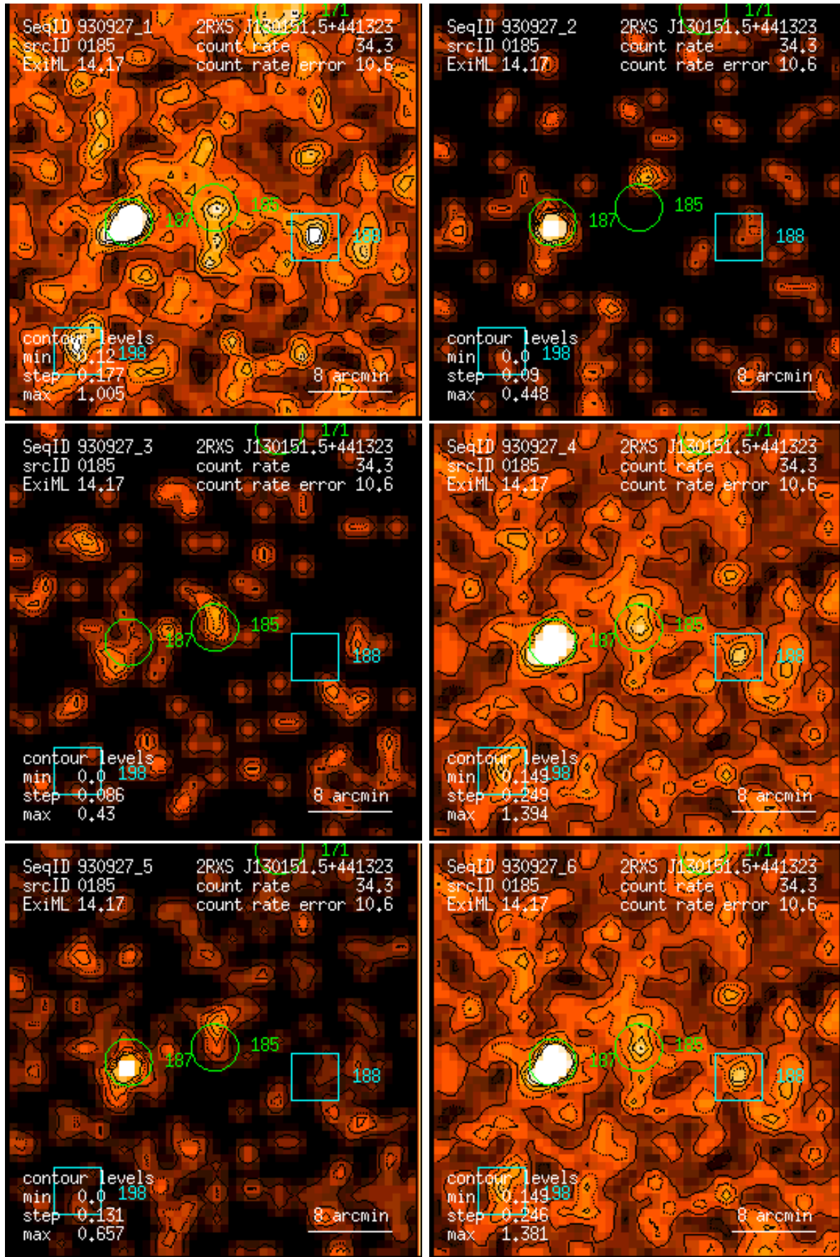
Figure 185: RASS 930927: detection 0185: band rate images, Gaussian filter: (1) PSPC channels 11 – 41, (2) 52 – 90, (3) 91 – 201, (4) 11 – 235, (5) 52 – 201, (6) 11 – 201. Broad band rates in counts/ks. Band rate contour levels in counts/ks/arcmin 2 .
