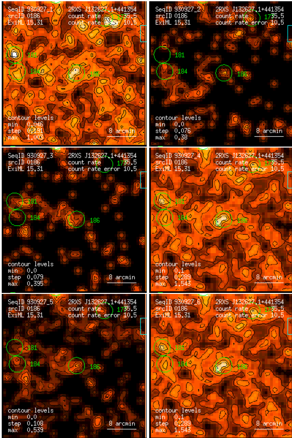
Figure 186: RASS 930927: detection 0186: band rate images, Gaussian filter: (1) PSPC channels 11 – 41, (2) 52 – 90, (3) 91 – 201, (4) 11 – 235, (5) 52 – 201, (6) 11 – 201. Broad band rates in counts/ks. Band rate contour levels in counts/ks/arcmin 2 .
