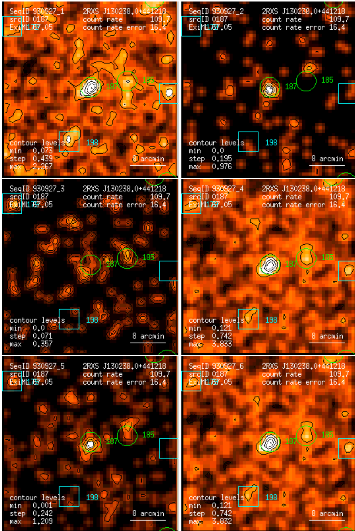
Figure 187: RASS 930927: detection 0187: band rate images, Gaussian filter: (1) PSPC channels 11 – 41, (2) 52 – 90, (3) 91 – 201, (4) 11 – 235, (5) 52 – 201, (6) 11 – 201. Broad band rates in counts/ks. Band rate contour levels in counts/ks/arcmin 2 .
