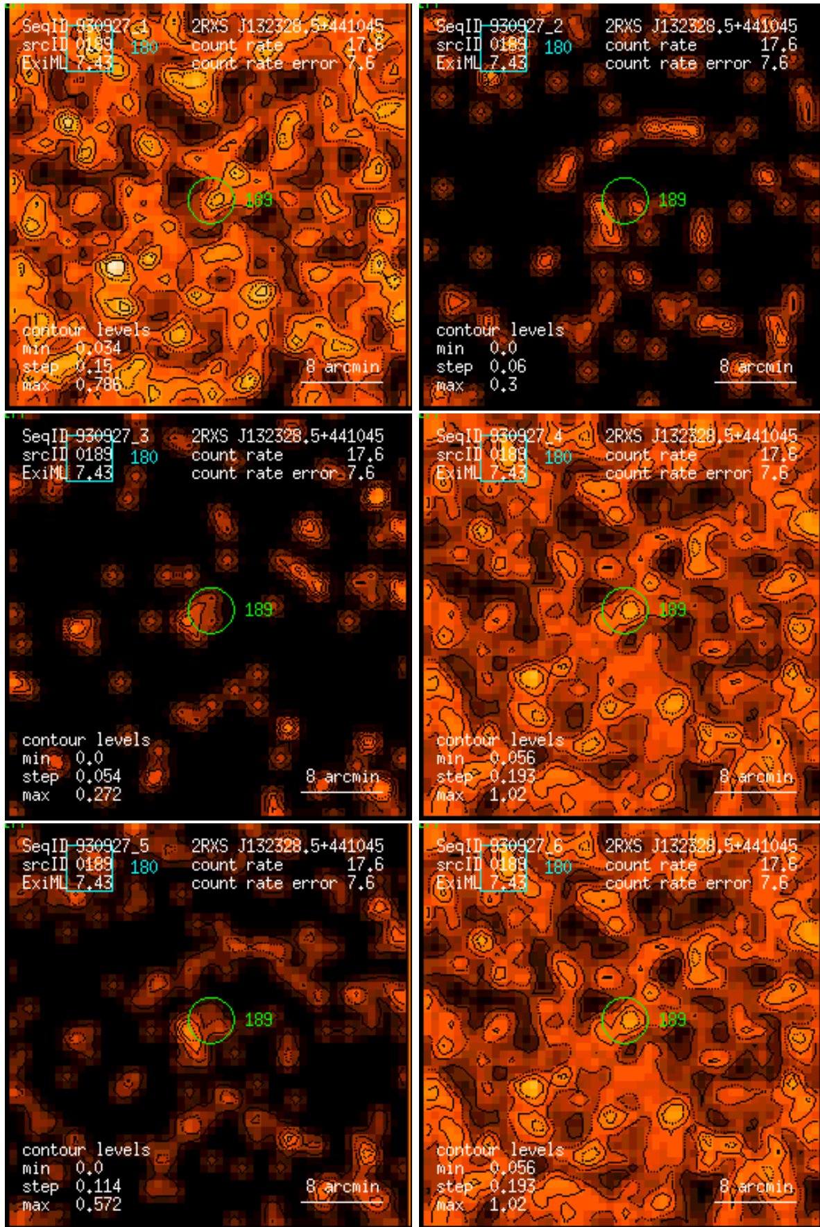
Figure 189: RASS 930927: detection 0189: band rate images, Gaussian filter: (1) PSPC channels 11 – 41, (2) 52 – 90, (3) 91 – 201, (4) 11 – 235, (5) 52 – 201, (6) 11 – 201. Broad band rates in counts/ks. Band rate contour levels in counts/ks/arcmin 2 .
