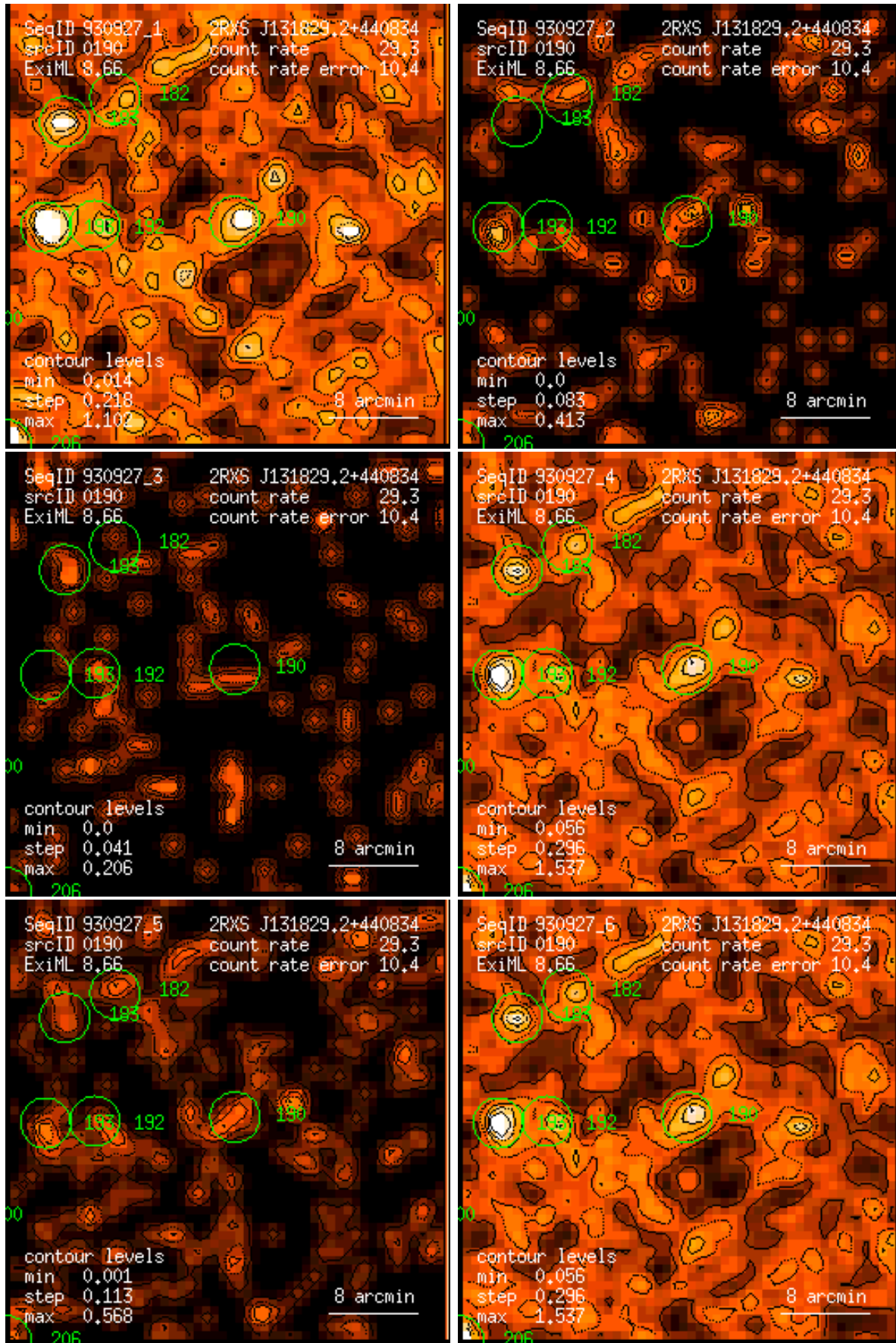
Figure 190: RASS 930927: detection 0190: band rate images, Gaussian filter: (1) PSPC channels 11 – 41, (2) 52 – 90, (3) 91 – 201, (4) 11 – 235, (5) 52 – 201, (6) 11 – 201. Broad band rates in counts/ks. Band rate contour levels in counts/ks/arcmin 2 .
