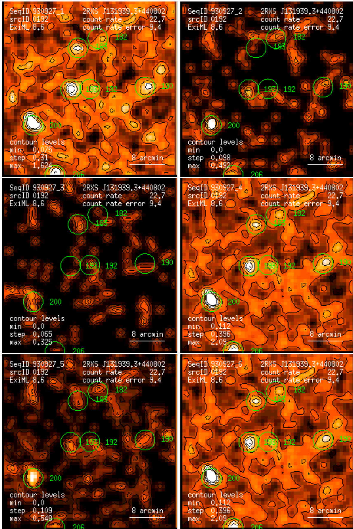
Figure 192: RASS 930927: detection 0192: band rate images, Gaussian filter: (1) PSPC channels 11 – 41, (2) 52 – 90, (3) 91 – 201, (4) 11 – 235, (5) 52 – 201, (6) 11 – 201. Broad band rates in counts/ks. Band rate contour levels in counts/ks/arcmin 2 .
