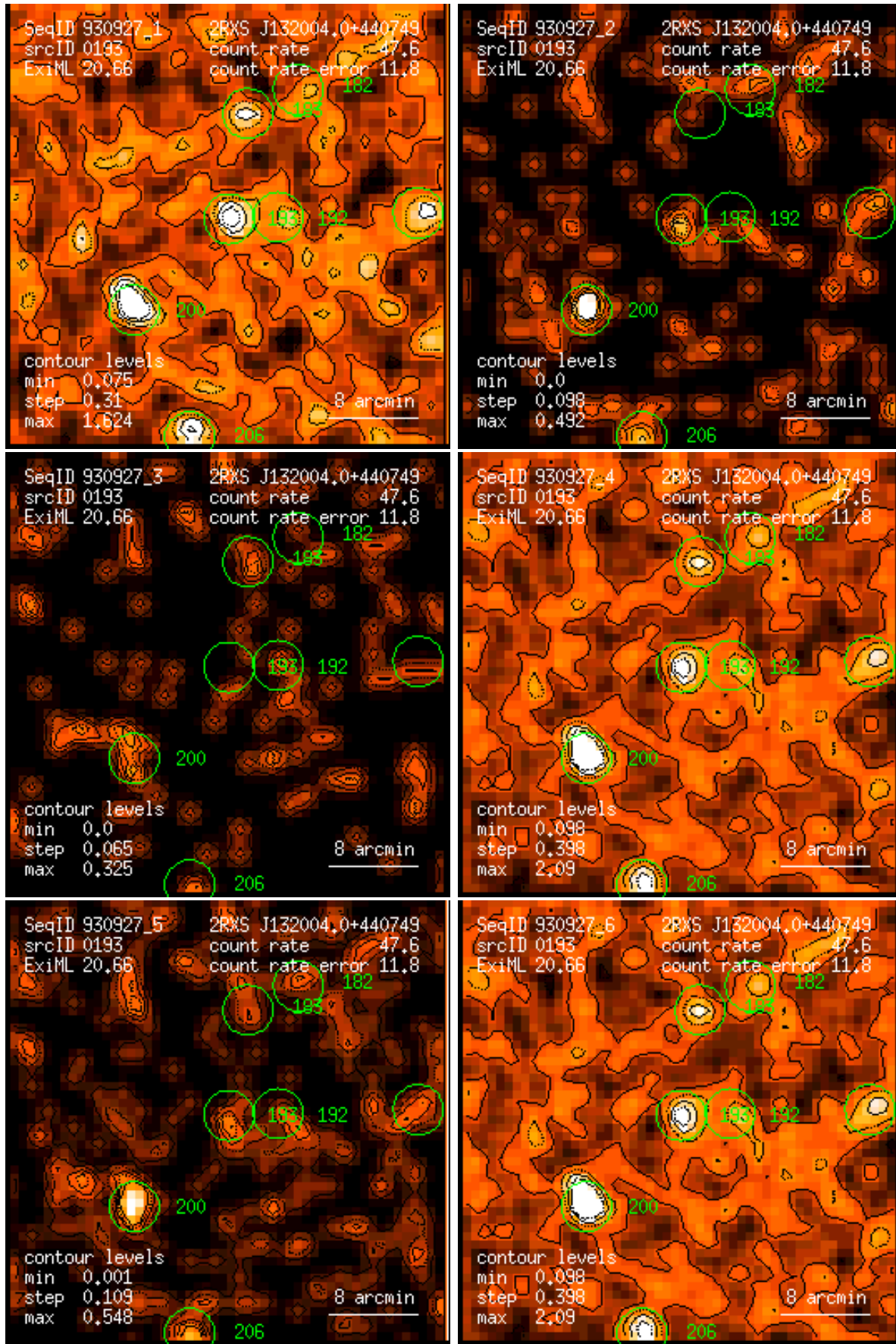
Figure 193: RASS 930927: detection 0193: band rate images, Gaussian filter: (1) PSPC channels 11 – 41, (2) 52 – 90, (3) 91 – 201, (4) 11 – 235, (5) 52 – 201, (6) 11 – 201. Broad band rates in counts/ks. Band rate contour levels in counts/ks/arcmin 2 .
