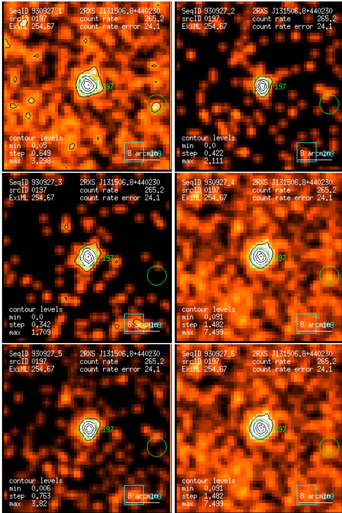
Figure 197: RASS 930927: detection 0197: band rate images, Gaussian filter: (1) PSPC channels 11 – 41, (2) 52 – 90, (3) 91 – 201, (4) 11 – 235, (5) 52 – 201, (6) 11 – 201. Broad band rates in counts/ks. Band rate contour levels in counts/ks/arcmin 2 .
