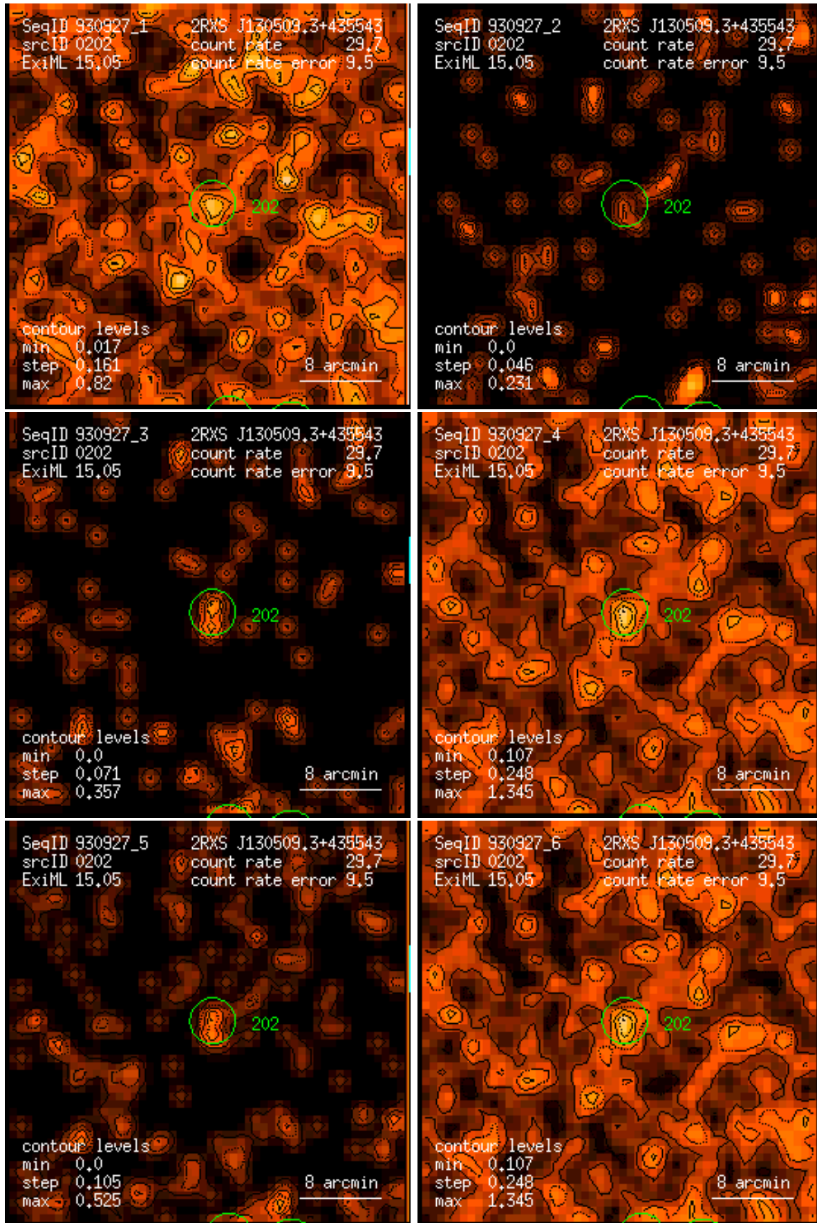
Figure 202: RASS 930927: detection 0202: band rate images, Gaussian filter: (1) PSPC channels 11 – 41, (2) 52 – 90, (3) 91 – 201, (4) 11 – 235, (5) 52 – 201, (6) 11 – 201. Broad band rates in counts/ks. Band rate contour levels in counts/ks/arcmin 2 .
