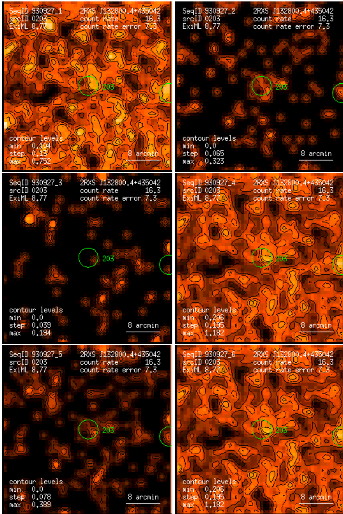
Figure 203: RASS 930927: detection 0203: band rate images, Gaussian filter: (1) PSPC channels 11 – 41, (2) 52 – 90, (3) 91 – 201, (4) 11 – 235, (5) 52 – 201, (6) 11 – 201. Broad band rates in counts/ks. Band rate contour levels in counts/ks/arcmin 2 .
