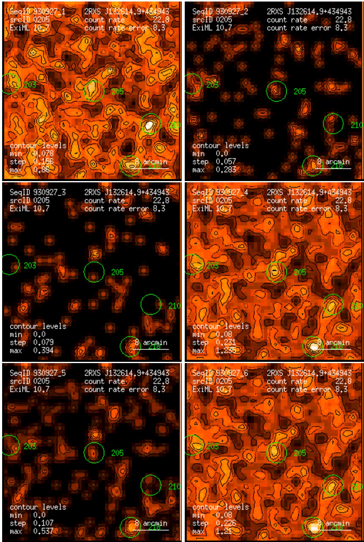
Figure 205: RASS 930927: detection 0205: band rate images, Gaussian filter: (1) PSPC channels 11 – 41, (2) 52 – 90, (3) 91 – 201, (4) 11 – 235, (5) 52 – 201, (6) 11 – 201. Broad band rates in counts/ks. Band rate contour levels in counts/ks/arcmin 2 .
