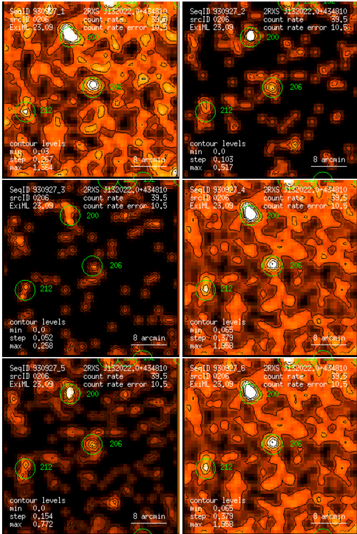
Figure 206: RASS 930927: detection 0206: band rate images, Gaussian filter: (1) PSPC channels 11 – 41, (2) 52 – 90, (3) 91 – 201, (4) 11 – 235, (5) 52 – 201, (6) 11 – 201. Broad band rates in counts/ks. Band rate contour levels in counts/ks/arcmin 2 .
