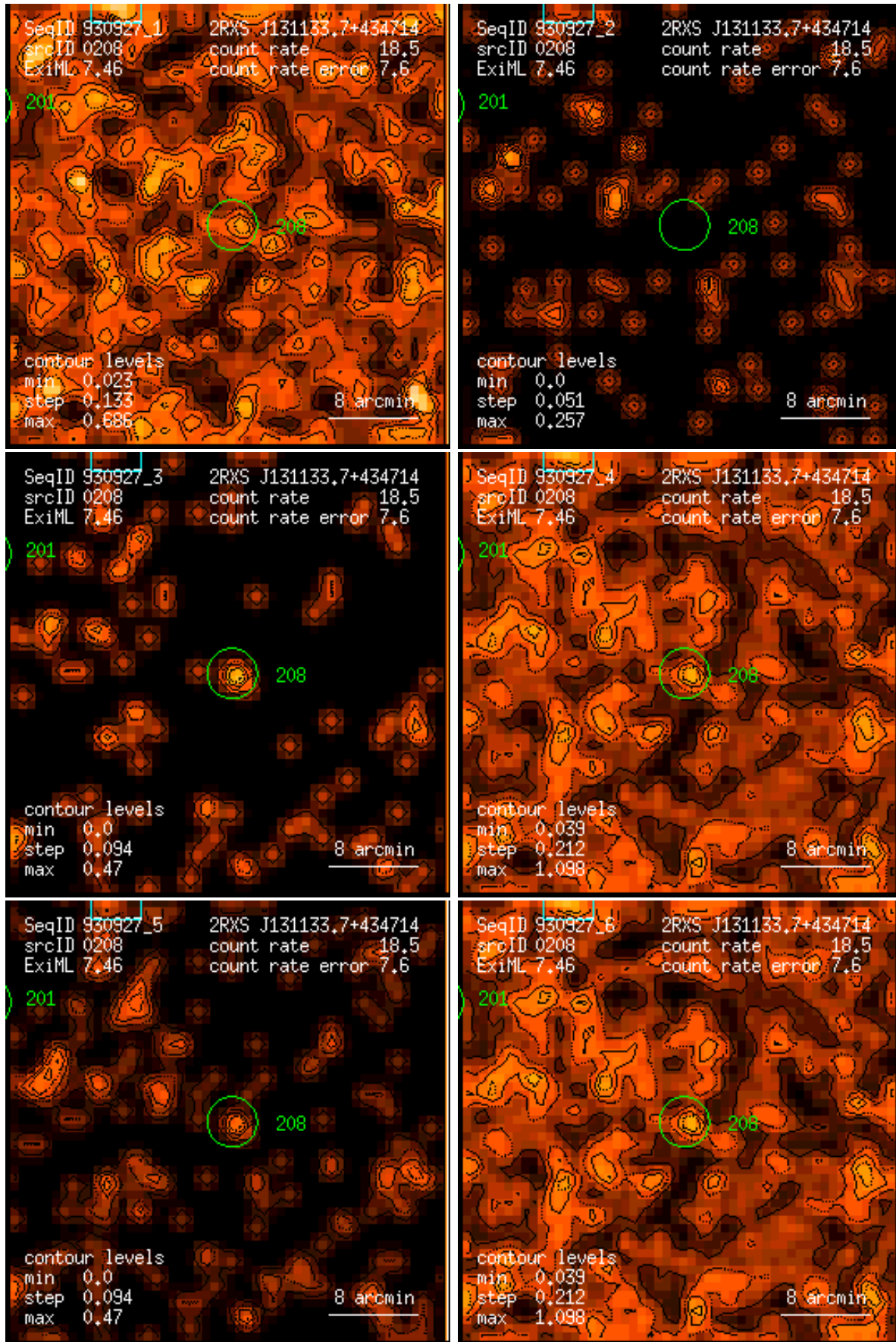
Figure 208: RASS 930927: detection 0208: band rate images, Gaussian filter: (1) PSPC channels 11 – 41, (2) 52 – 90, (3) 91 – 201, (4) 11 – 235, (5) 52 – 201, (6) 11 – 201. Broad band rates in counts/ks. Band rate contour levels in counts/ks/arcmin 2 .
