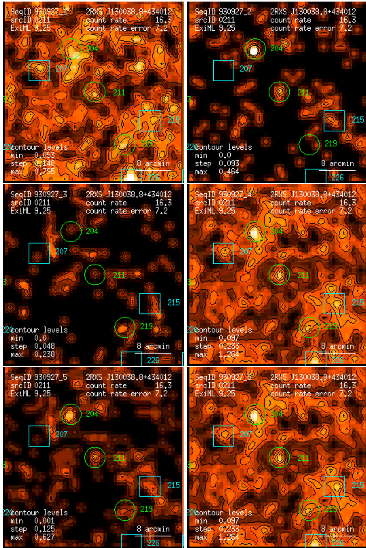
Figure 211: RASS 930927: detection 0211: band rate images, Gaussian filter: (1) PSPC channels 11 – 41, (2) 52 – 90, (3) 91 – 201, (4) 11 – 235, (5) 52 – 201, (6) 11 – 201. Broad band rates in counts/ks. Band rate contour levels in counts/ks/arcmin 2 .
