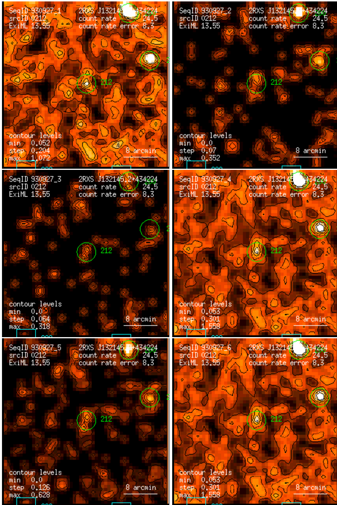
Figure 212: RASS 930927: detection 0212: band rate images, Gaussian filter: (1) PSPC channels 11 – 41, (2) 52 – 90, (3) 91 – 201, (4) 11 – 235, (5) 52 – 201, (6) 11 – 201. Broad band rates in counts/ks. Band rate contour levels in counts/ks/arcmin 2 .
