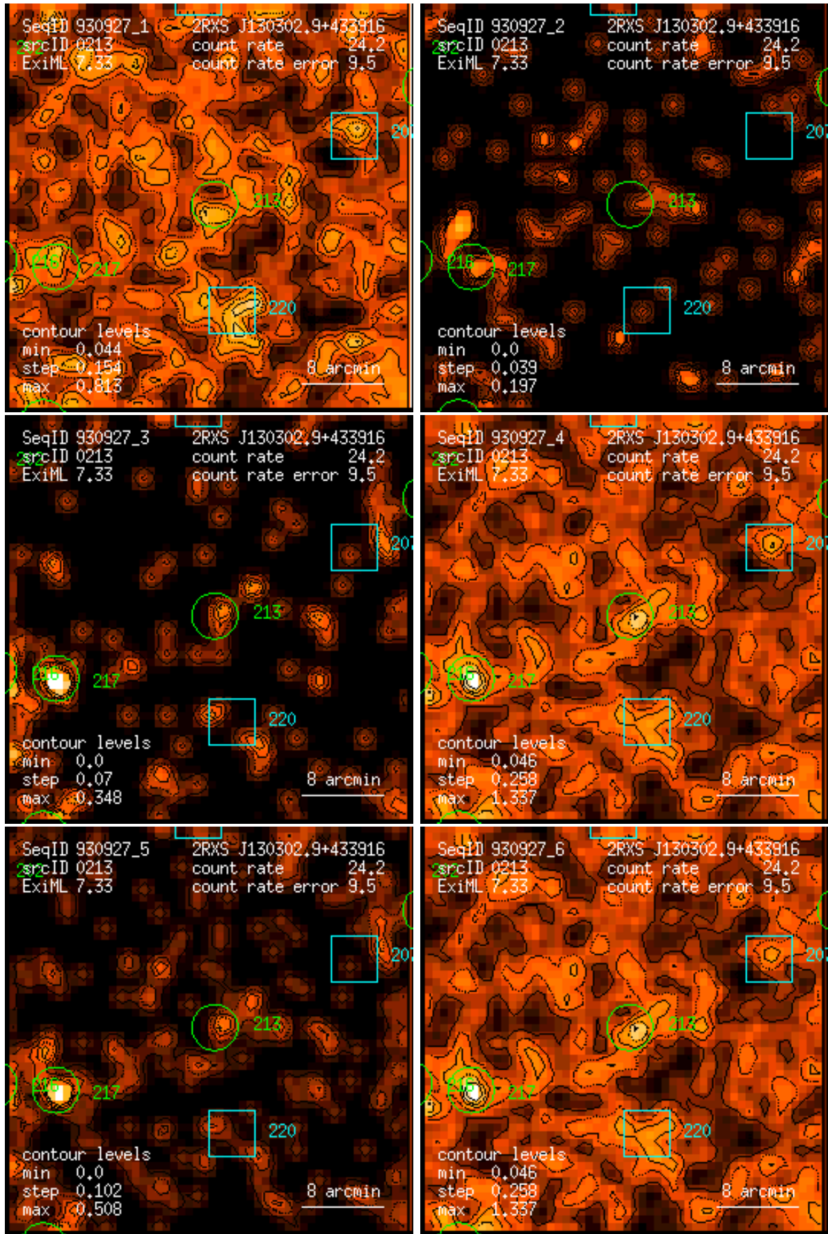
Figure 213: RASS 930927: detection 0213: band rate images, Gaussian filter: (1) PSPC channels 11 – 41, (2) 52 – 90, (3) 91 – 201, (4) 11 – 235, (5) 52 – 201, (6) 11 – 201. Broad band rates in counts/ks. Band rate contour levels in counts/ks/arcmin 2 .
