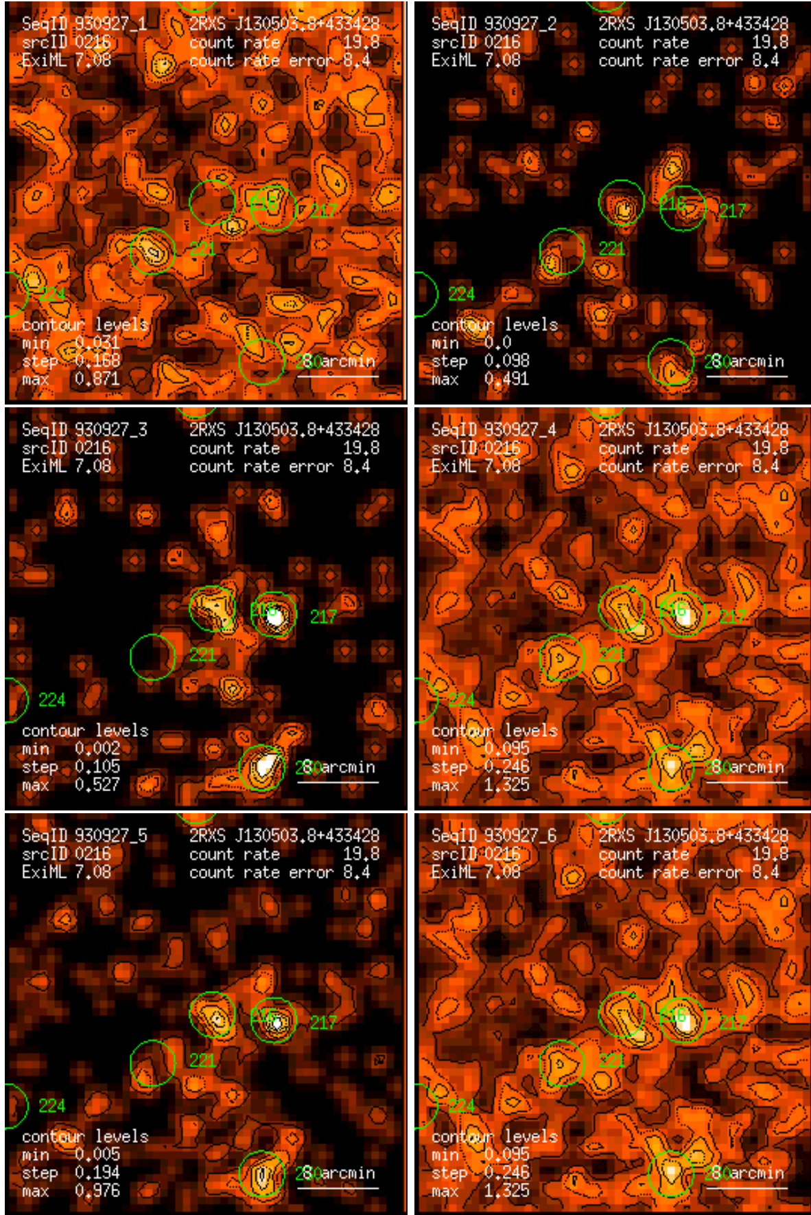
Figure 216: RASS 930927: detection 0216: band rate images, Gaussian filter: (1) PSPC channels 11 – 41, (2) 52 – 90, (3) 91 – 201, (4) 11 – 235, (5) 52 – 201, (6) 11 – 201. Broad band rates in counts/ks. Band rate contour levels in counts/ks/arcmin 2 .
