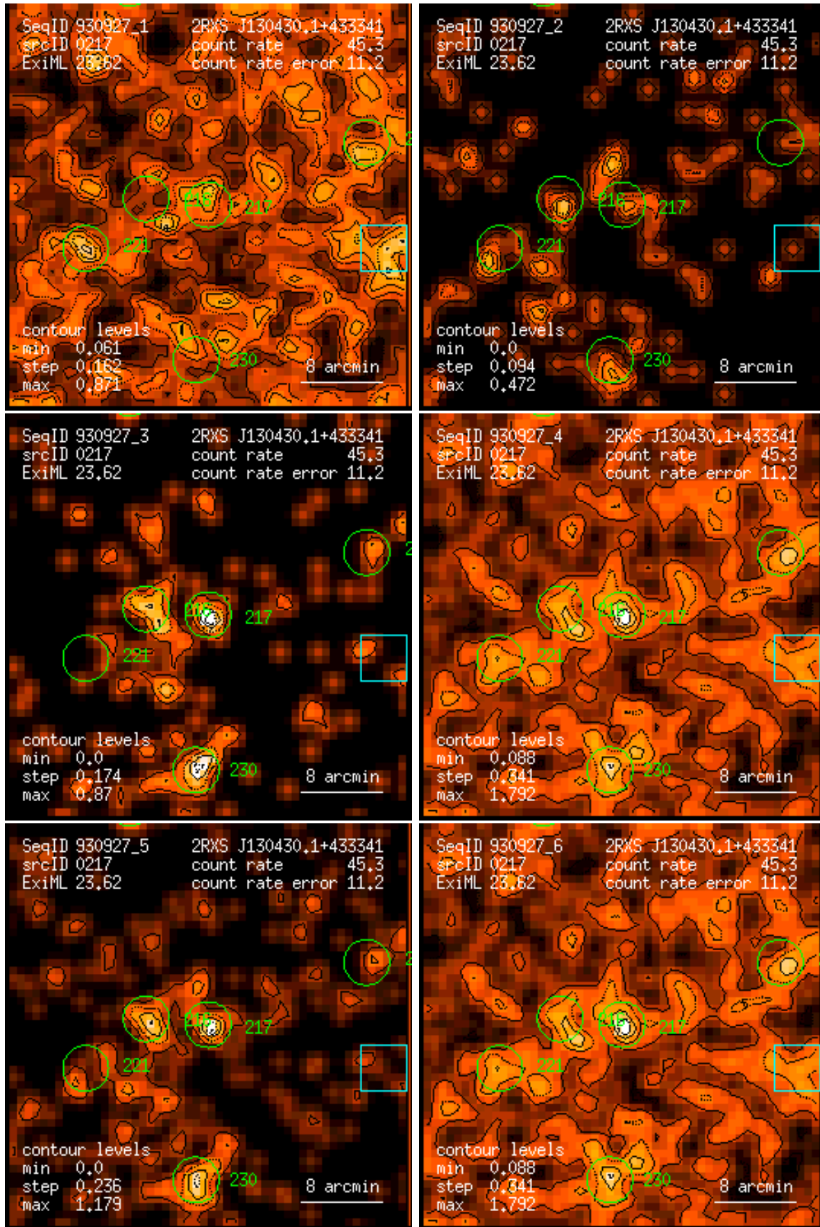
Figure 217: RASS 930927: detection 0217: band rate images, Gaussian filter: (1) PSPC channels 11 – 41, (2) 52 – 90, (3) 91 – 201, (4) 11 – 235, (5) 52 – 201, (6) 11 – 201. Broad band rates in counts/ks. Band rate contour levels in counts/ks/arcmin 2 .
