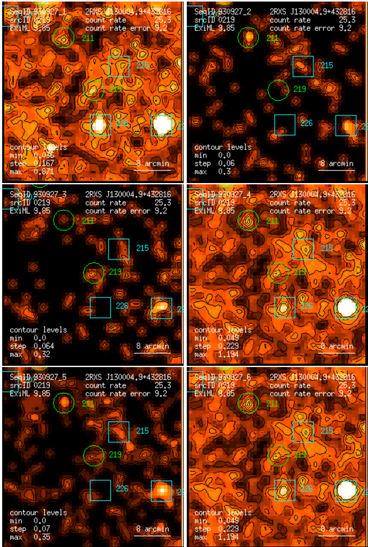
Figure 219: RASS 930927: detection 0219: band rate images, Gaussian filter: (1) PSPC channels 11 – 41, (2) 52 – 90, (3) 91 – 201, (4) 11 – 235, (5) 52 – 201, (6) 11 – 201. Broad band rates in counts/ks. Band rate contour levels in counts/ks/arcmin 2 .
