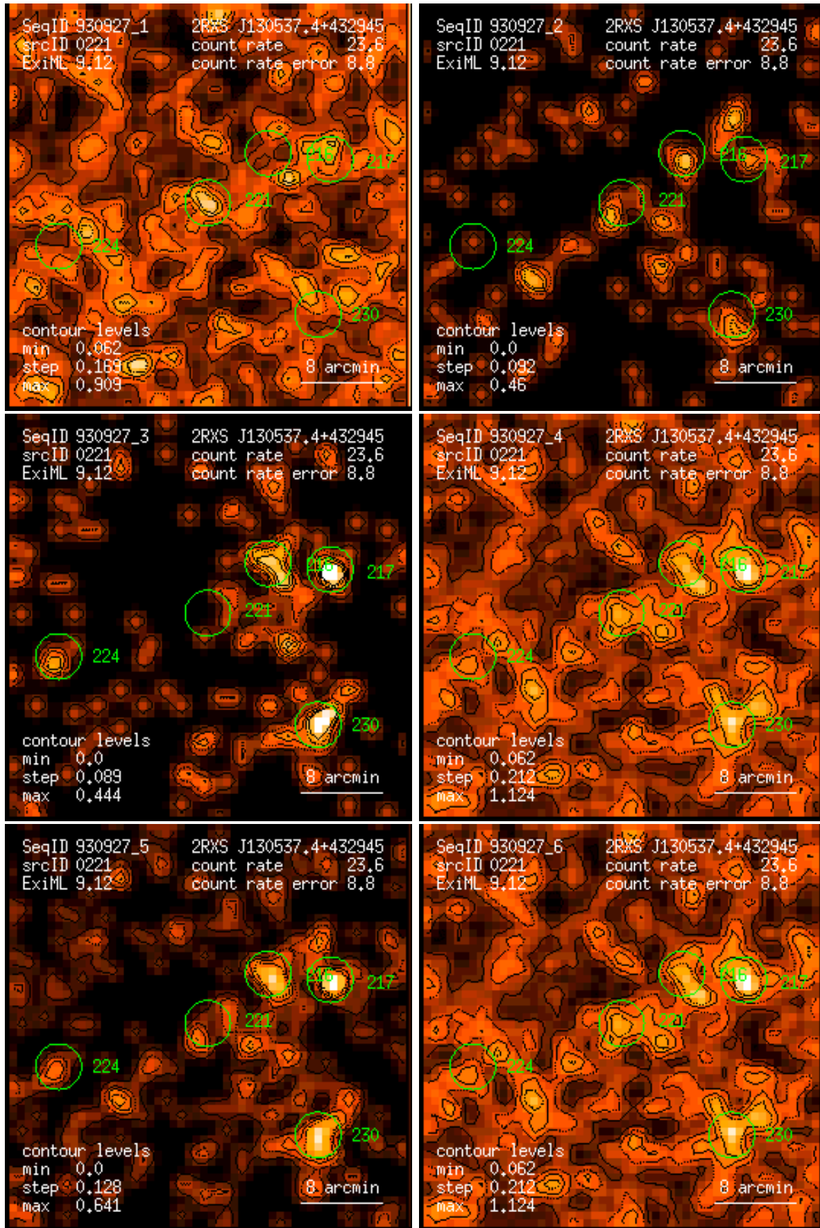
Figure 221: RASS 930927: detection 0221: band rate images, Gaussian filter: (1) PSPC channels 11 – 41, (2) 52 – 90, (3) 91 – 201, (4) 11 – 235, (5) 52 – 201, (6) 11 – 201. Broad band rates in counts/ks. Band rate contour levels in counts/ks/arcmin 2 .
