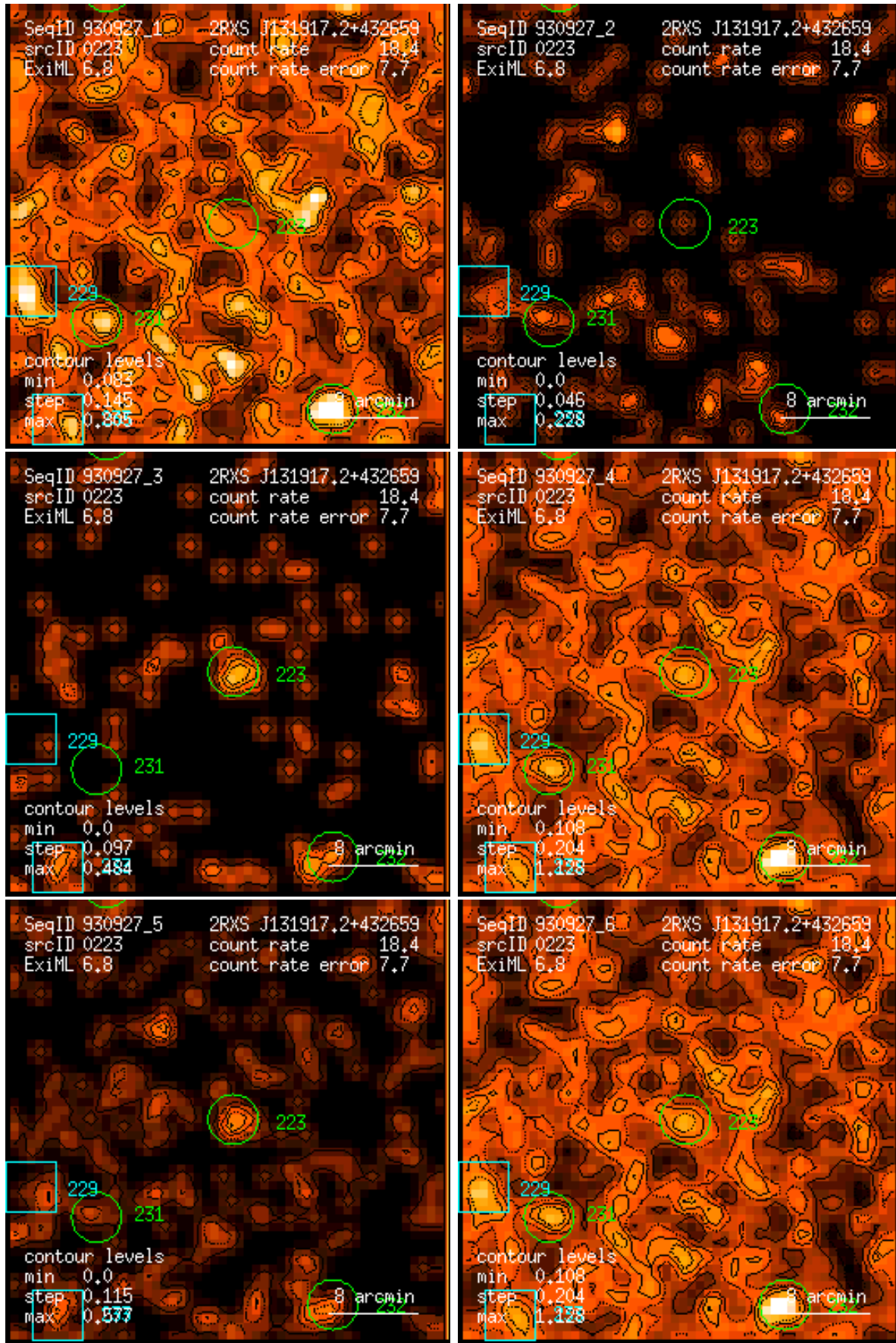
Figure 223: RASS 930927: detection 0223: band rate images, Gaussian filter: (1) PSPC channels 11 – 41, (2) 52 – 90, (3) 91 – 201, (4) 11 – 235, (5) 52 – 201, (6) 11 – 201. Broad band rates in counts/ks. Band rate contour levels in counts/ks/arcmin 2 .
