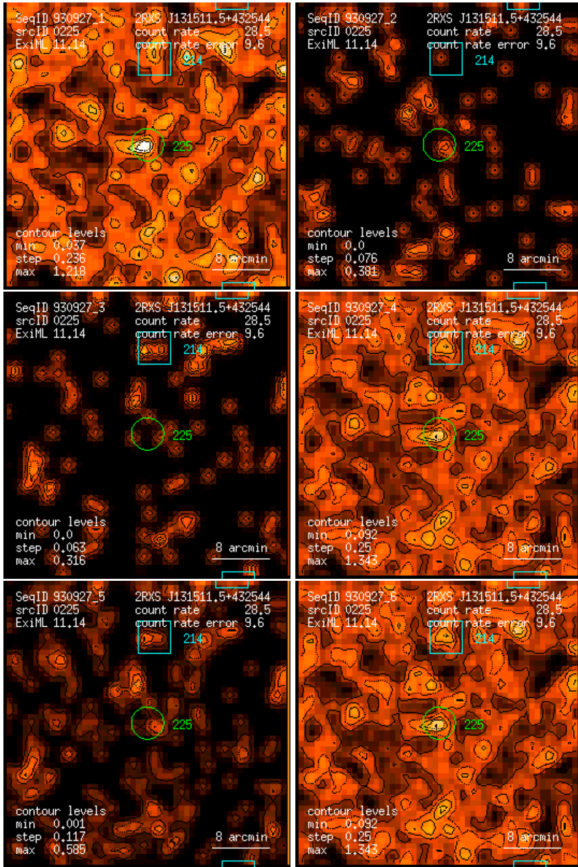
Figure 225: RASS 930927: detection 0225: band rate images, Gaussian filter: (1) PSPC channels 11 – 41, (2) 52 – 90, (3) 91 – 201, (4) 11 – 235, (5) 52 – 201, (6) 11 – 201. Broad band rates in counts/ks. Band rate contour levels in counts/ks/arcmin 2 .
