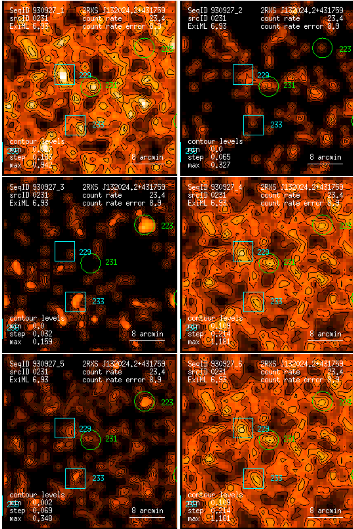
Figure 231: RASS 930927: detection 0231: band rate images, Gaussian filter: (1) PSPC channels 11 – 41, (2) 52 – 90, (3) 91 – 201, (4) 11 – 235, (5) 52 – 201, (6) 11 – 201. Broad band rates in counts/ks. Band rate contour levels in counts/ks/arcmin 2 .
