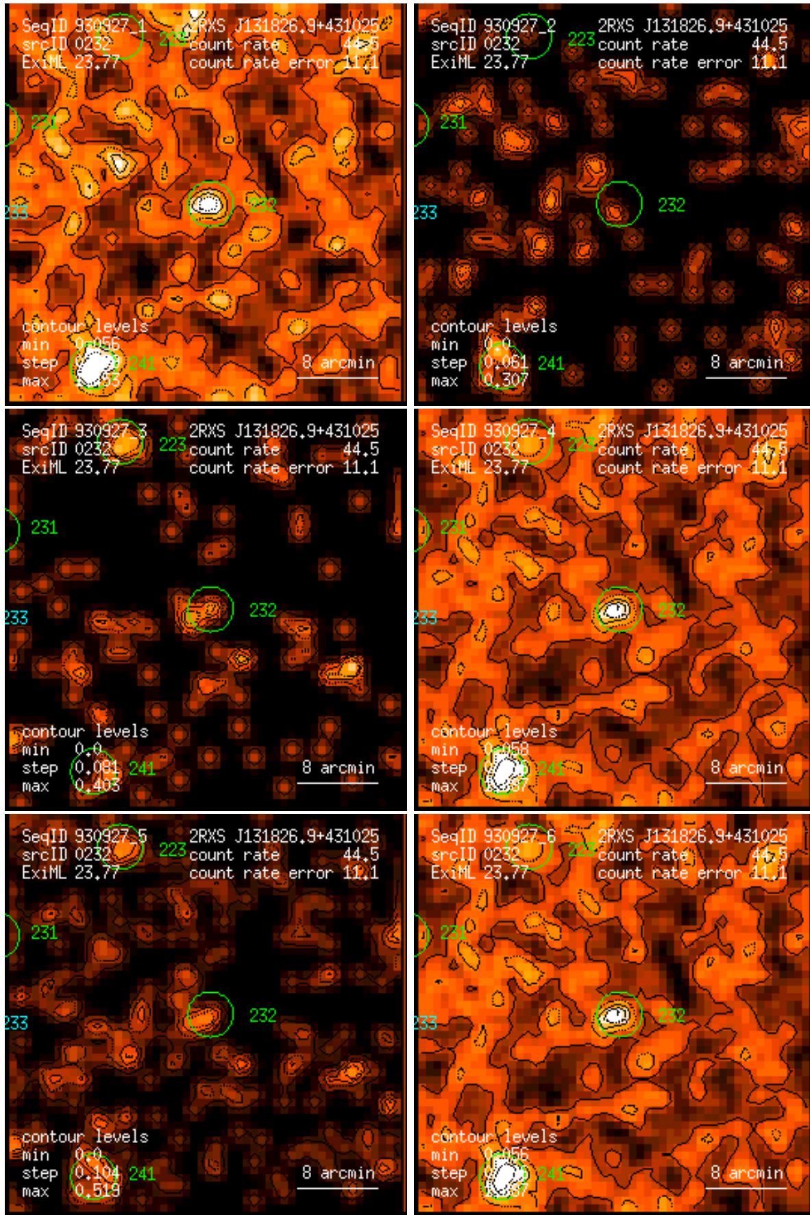
Figure 232: RASS 930927: detection 0232: band rate images, Gaussian filter: (1) PSPC channels 11 – 41, (2) 52 – 90, (3) 91 – 201, (4) 11 – 235, (5) 52 – 201, (6) 11 – 201. Broad band rates in counts/ks. Band rate contour levels in counts/ks/arcmin 2 .
