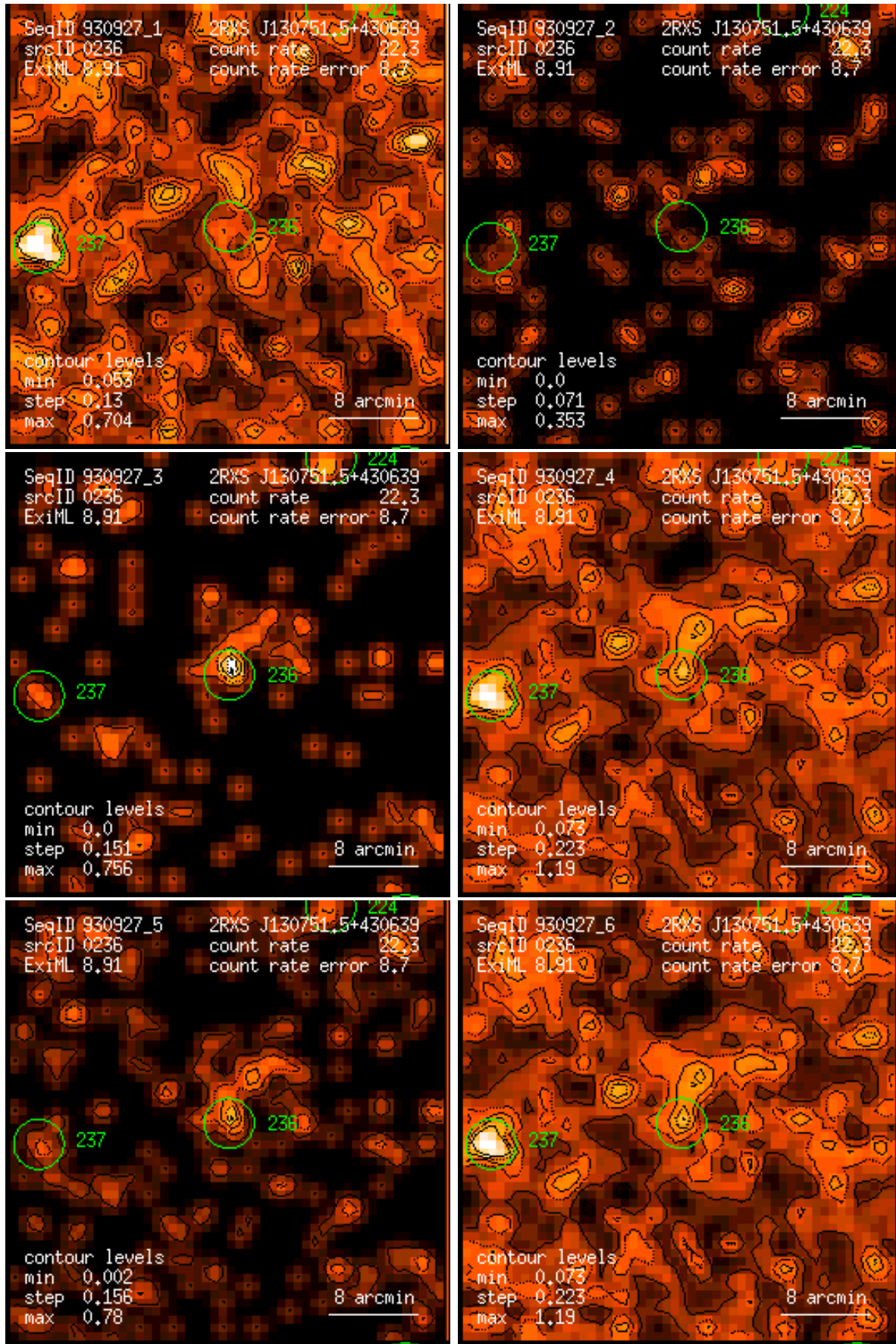
Figure 236: RASS 930927: detection 0236: band rate images, Gaussian filter: (1) PSPC channels 11 – 41, (2) 52 – 90, (3) 91 – 201, (4) 11 – 235, (5) 52 – 201, (6) 11 – 201. Broad band rates in counts/ks. Band rate contour levels in counts/ks/arcmin 2 .
