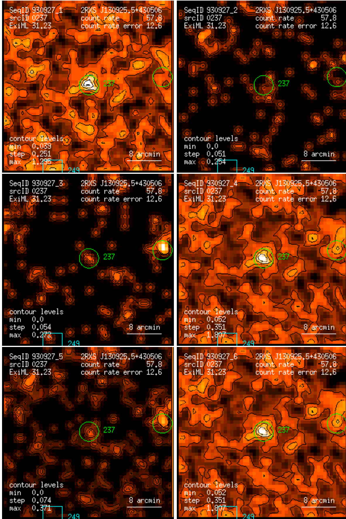
Figure 237: RASS 930927: detection 0237: band rate images, Gaussian filter: (1) PSPC channels 11 – 41, (2) 52 – 90, (3) 91 – 201, (4) 11 – 235, (5) 52 – 201, (6) 11 – 201. Broad band rates in counts/ks. Band rate contour levels in counts/ks/arcmin 2 .
