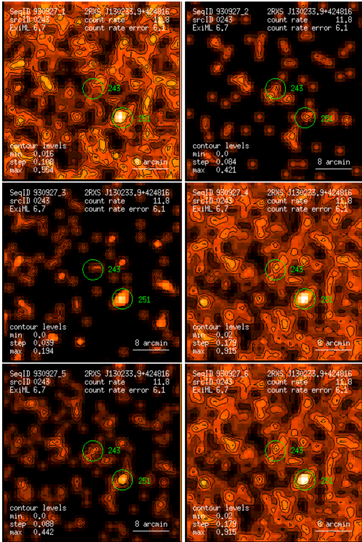
Figure 243: RASS 930927: detection 0243: band rate images, Gaussian filter: (1) PSPC channels 11 – 41, (2) 52 – 90, (3) 91 – 201, (4) 11 – 235, (5) 52 – 201, (6) 11 – 201. Broad band rates in counts/ks. Band rate contour levels in counts/ks/arcmin 2 .
