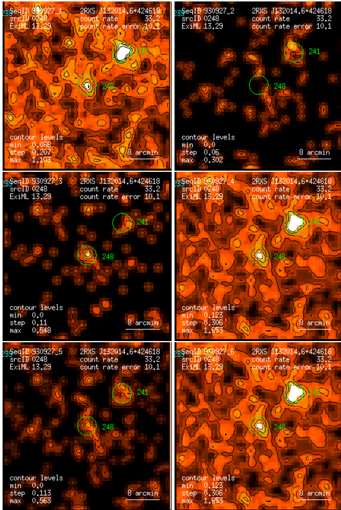
Figure 248: RASS 930927: detection 0248: band rate images, Gaussian filter: (1) PSPC channels 11 – 41, (2) 52 – 90, (3) 91 – 201, (4) 11 – 235, (5) 52 – 201, (6) 11 – 201. Broad band rates in counts/ks. Band rate contour levels in counts/ks/arcmin 2 .
