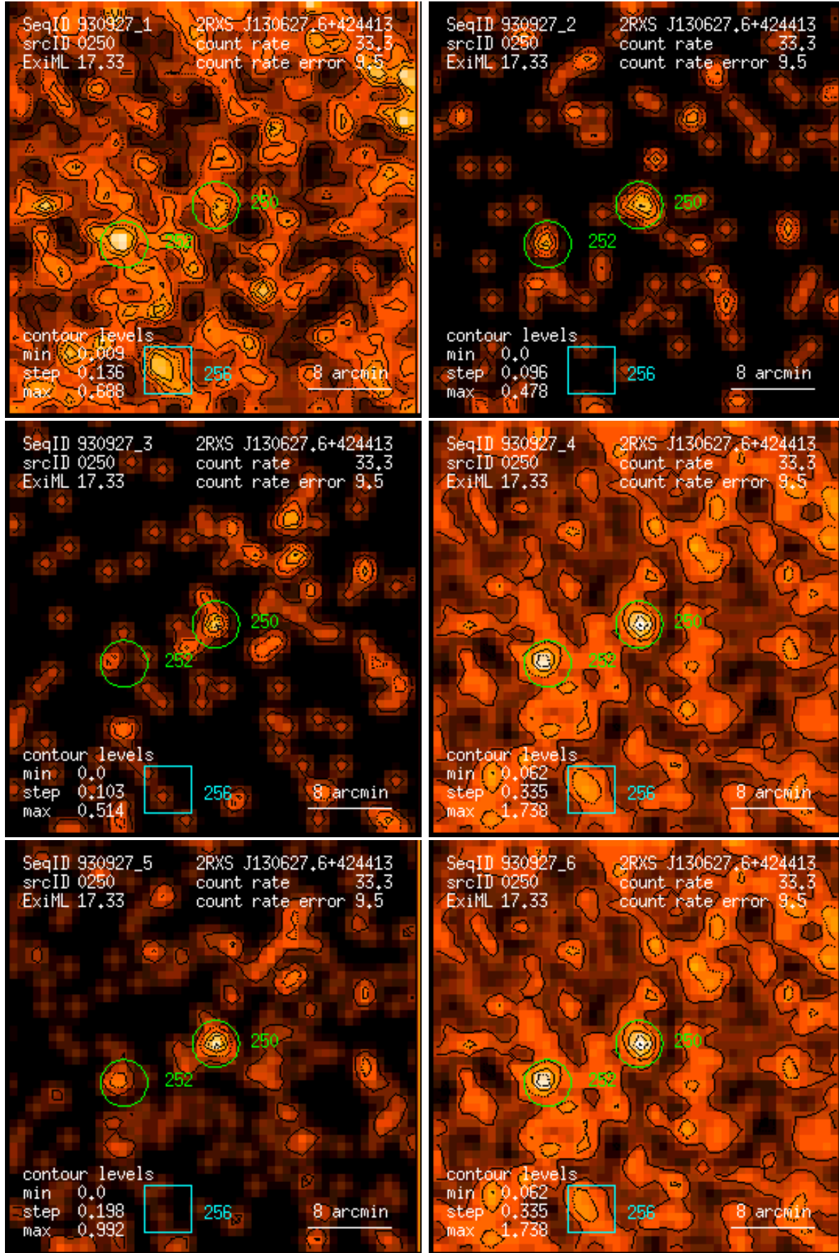
Figure 250: RASS 930927: detection 0250: band rate images, Gaussian filter: (1) PSPC channels 11 – 41, (2) 52 – 90, (3) 91 – 201, (4) 11 – 235, (5) 52 – 201, (6) 11 – 201. Broad band rates in counts/ks. Band rate contour levels in counts/ks/arcmin 2 .
