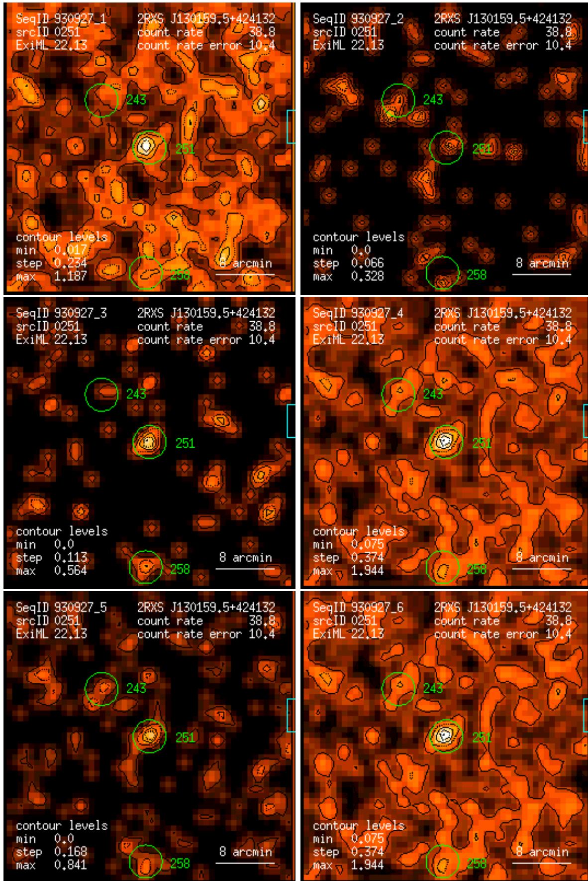
Figure 251: RASS 930927: detection 0251: band rate images, Gaussian filter: (1) PSPC channels 11 – 41, (2) 52 – 90, (3) 91 – 201, (4) 11 – 235, (5) 52 – 201, (6) 11 – 201. Broad band rates in counts/ks. Band rate contour levels in counts/ks/arcmin 2 .
